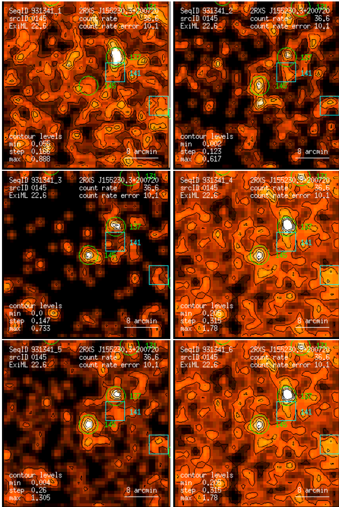
Figure 145: RASS 931341: detection 0145: band rate images, Gaussian filter: (1) PSPC channels 11 – 41, (2) 52 – 90, (3) 91 – 201, (4) 11 – 235, (5) 52 – 201, (6) 11 – 201. Broad band rates in counts/ks. Band rate contour levels in counts/ks/arcmin 2 .
