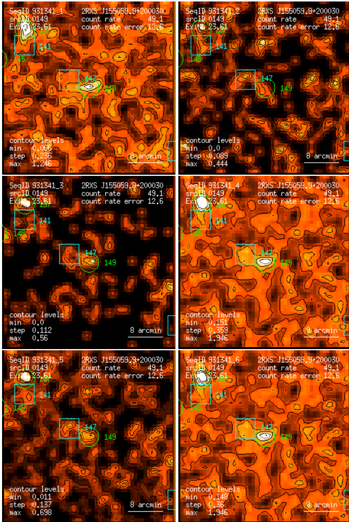
Figure 149: RASS 931341: detection 0149: band rate images, Gaussian filter: (1) PSPC channels 11 – 41, (2) 52 – 90, (3) 91 – 201, (4) 11 – 235, (5) 52 – 201, (6) 11 – 201. Broad band rates in counts/ks. Band rate contour levels in counts/ks/arcmin 2 .
