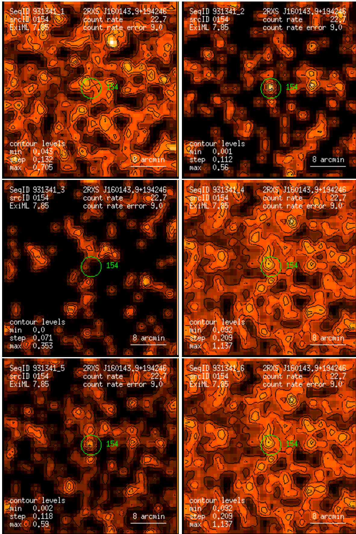
Figure 154: RASS 931341: detection 0154: band rate images, Gaussian filter: (1) PSPC channels 11 – 41, (2) 52 – 90, (3) 91 – 201, (4) 11 – 235, (5) 52 – 201, (6) 11 – 201. Broad band rates in counts/ks. Band rate contour levels in counts/ks/arcmin 2 .
