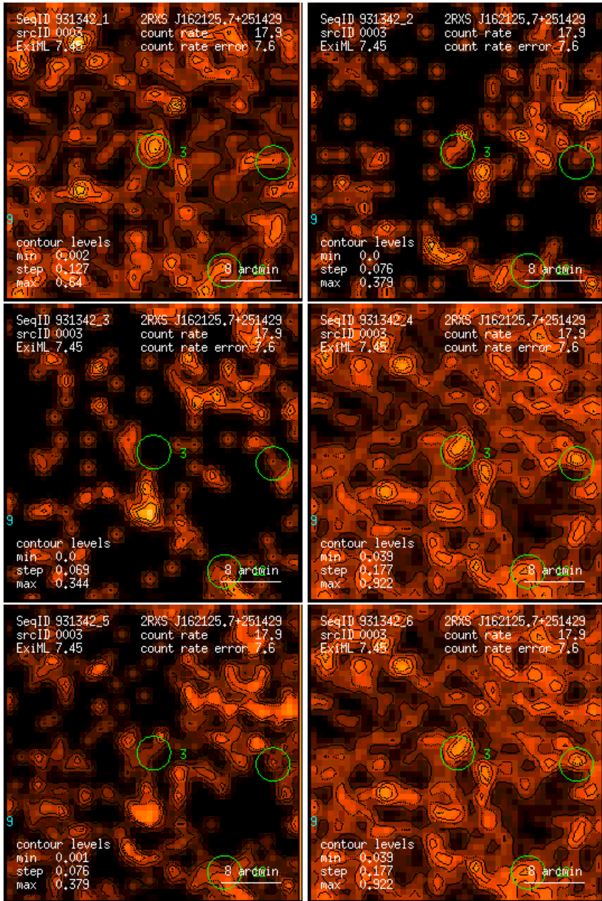
Figure 3: RASS 931342: detection 0003: band rate images, Gaussian filter: (1) PSPC channels 11 – 41, (2) 52 – 90, (3) 91 – 201, (4) 11 – 235, (5) 52 – 201, (6) 11 – 201. Broad band rates in counts/ks. Band rate contour levels in counts/ks/arcmin 2 .
