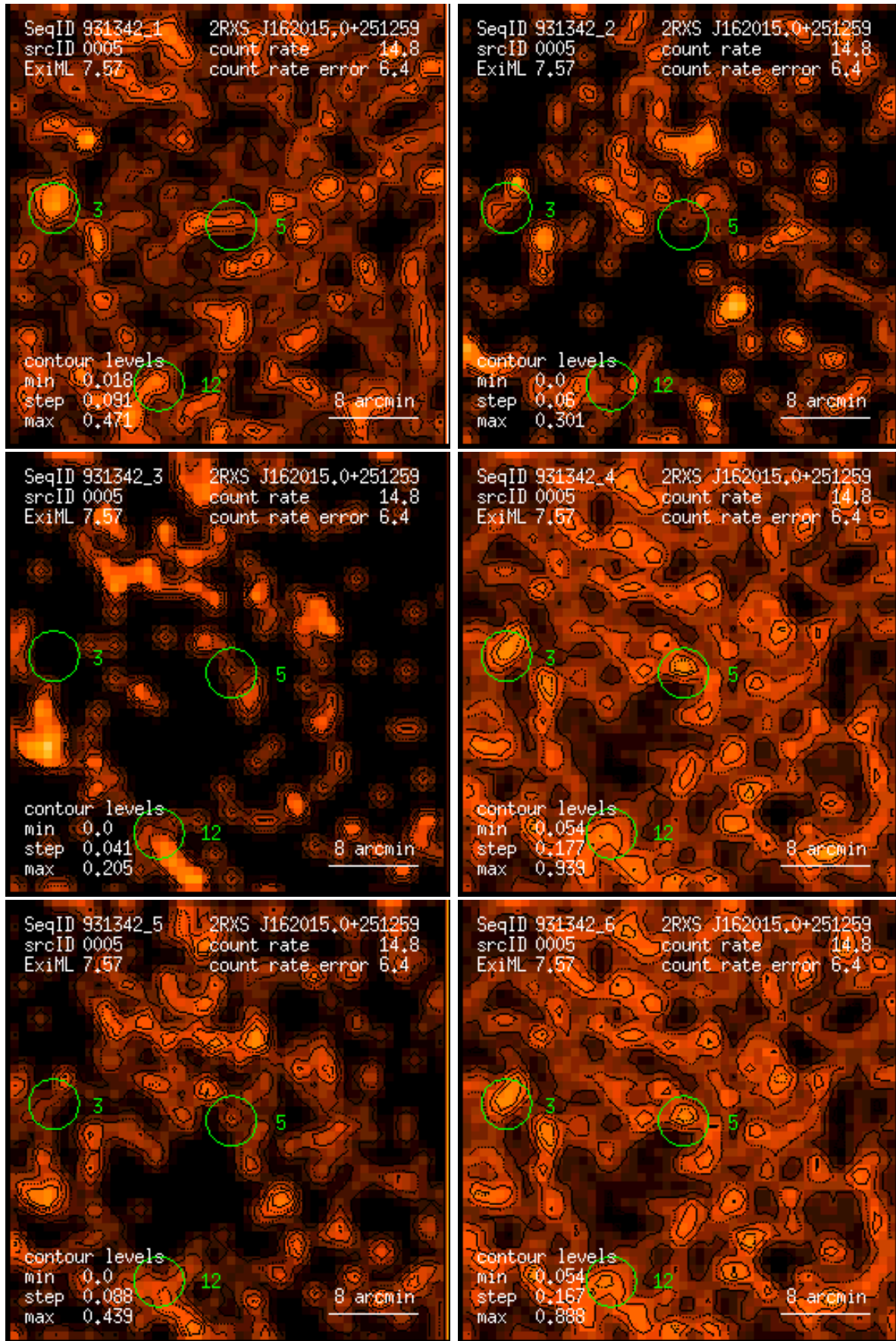
Figure 5: RASS 931342: detection 0005: band rate images, Gaussian filter: (1) PSPC channels 11 – 41, (2) 52 – 90, (3) 91 – 201, (4) 11 – 235, (5) 52 – 201, (6) 11 – 201. Broad band rates in counts/ks. Band rate contour levels in counts/ks/arcmin 2 .
