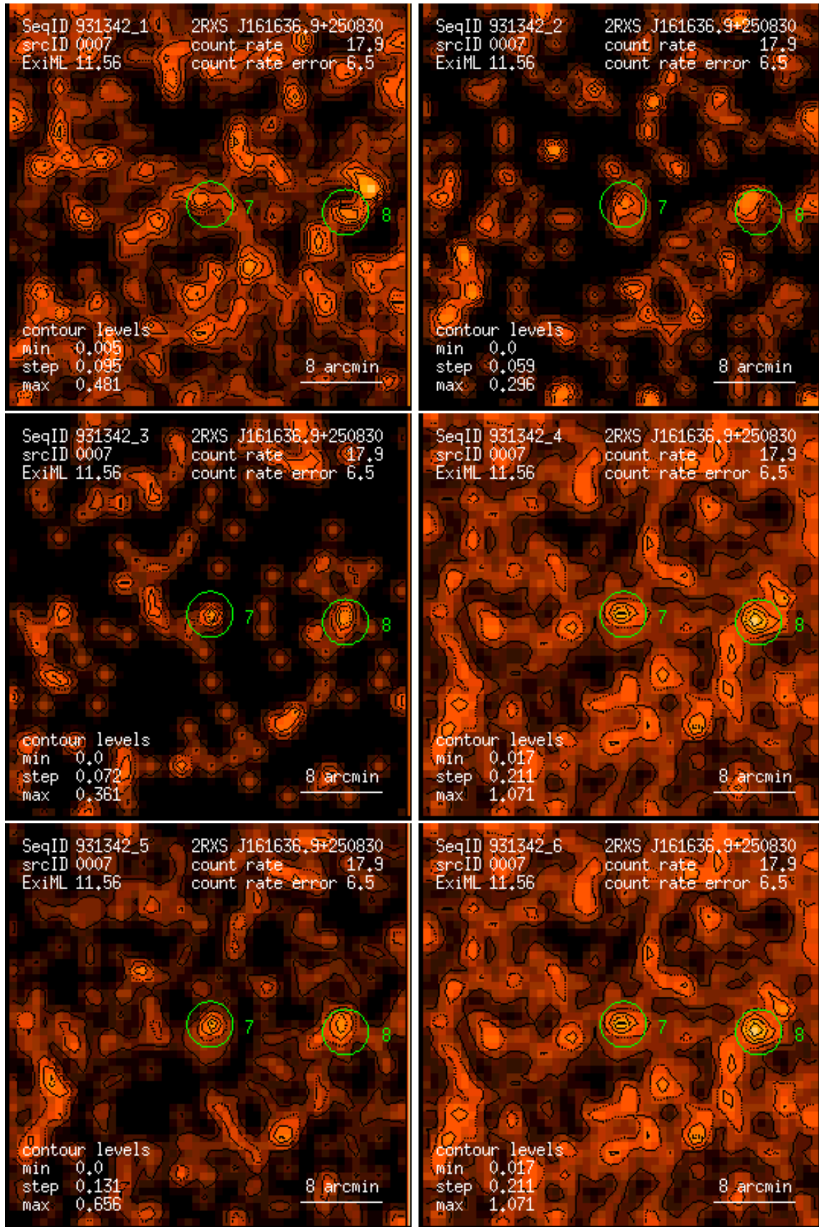
Figure 7: RASS 931342: detection 0007: band rate images, Gaussian filter: (1) PSPC channels 11 – 41, (2) 52 – 90, (3) 91 – 201, (4) 11 – 235, (5) 52 – 201, (6) 11 – 201. Broad band rates in counts/ks. Band rate contour levels in counts/ks/arcmin 2 .
