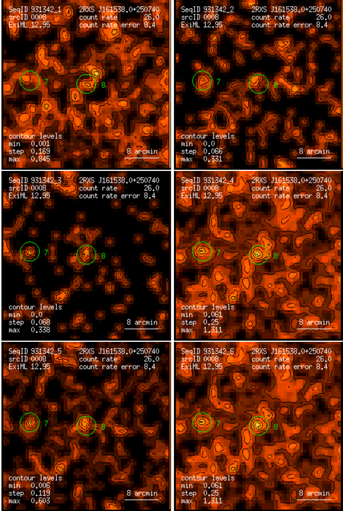
Figure 8: RASS 931342: detection 0008: band rate images, Gaussian filter: (1) PSPC channels 11 – 41, (2) 52 – 90, (3) 91 – 201, (4) 11 – 235, (5) 52 – 201, (6) 11 – 201. Broad band rates in counts/ks. Band rate contour levels in counts/ks/arcmin 2 .
