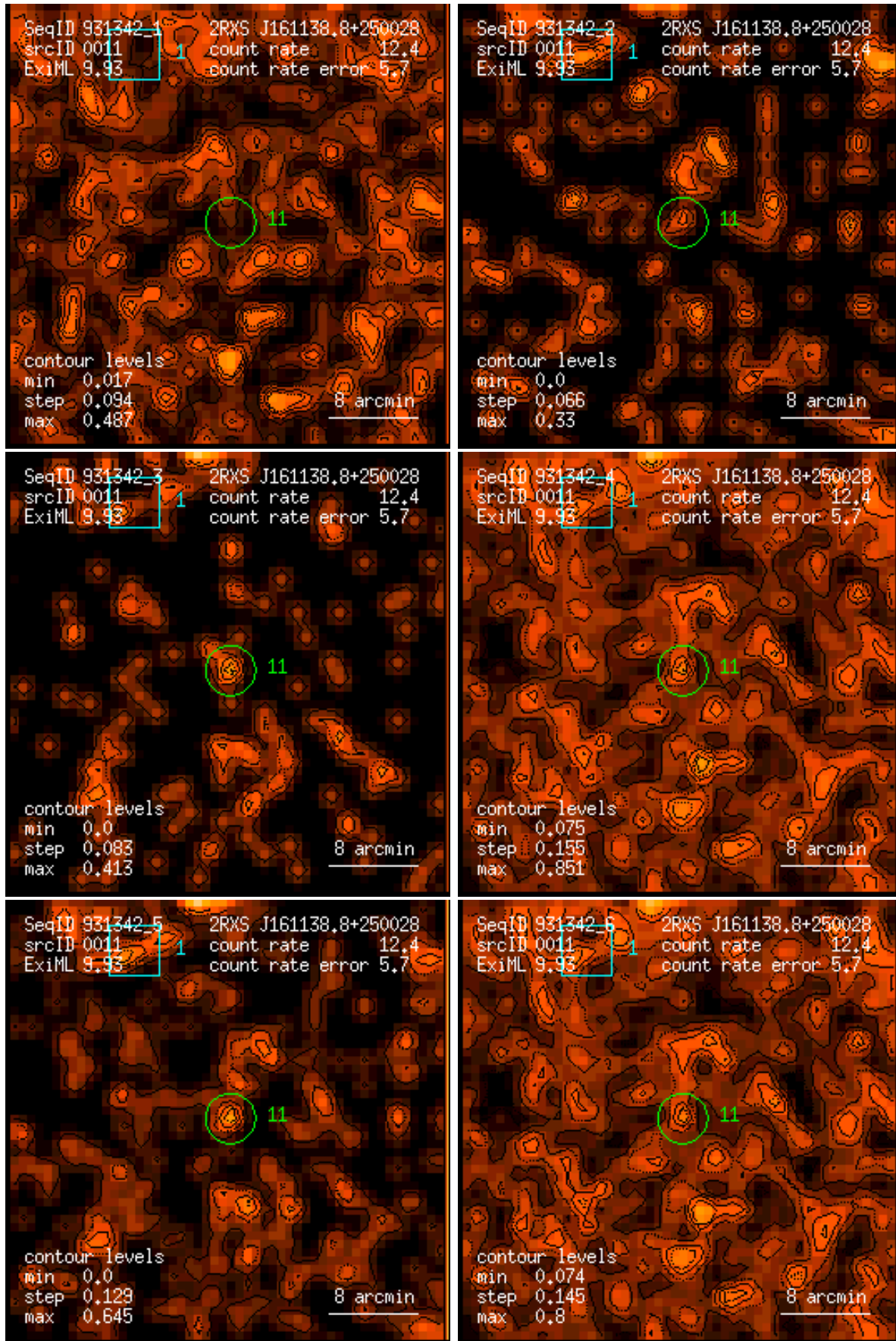
Figure 11: RASS 931342: detection 0011: band rate images, Gaussian filter: (1) PSPC channels 11 – 41, (2) 52 – 90, (3) 91 – 201, (4) 11 – 235, (5) 52 – 201, (6) 11 – 201. Broad band rates in counts/ks. Band rate contour levels in counts/ks/arcmin 2 .
