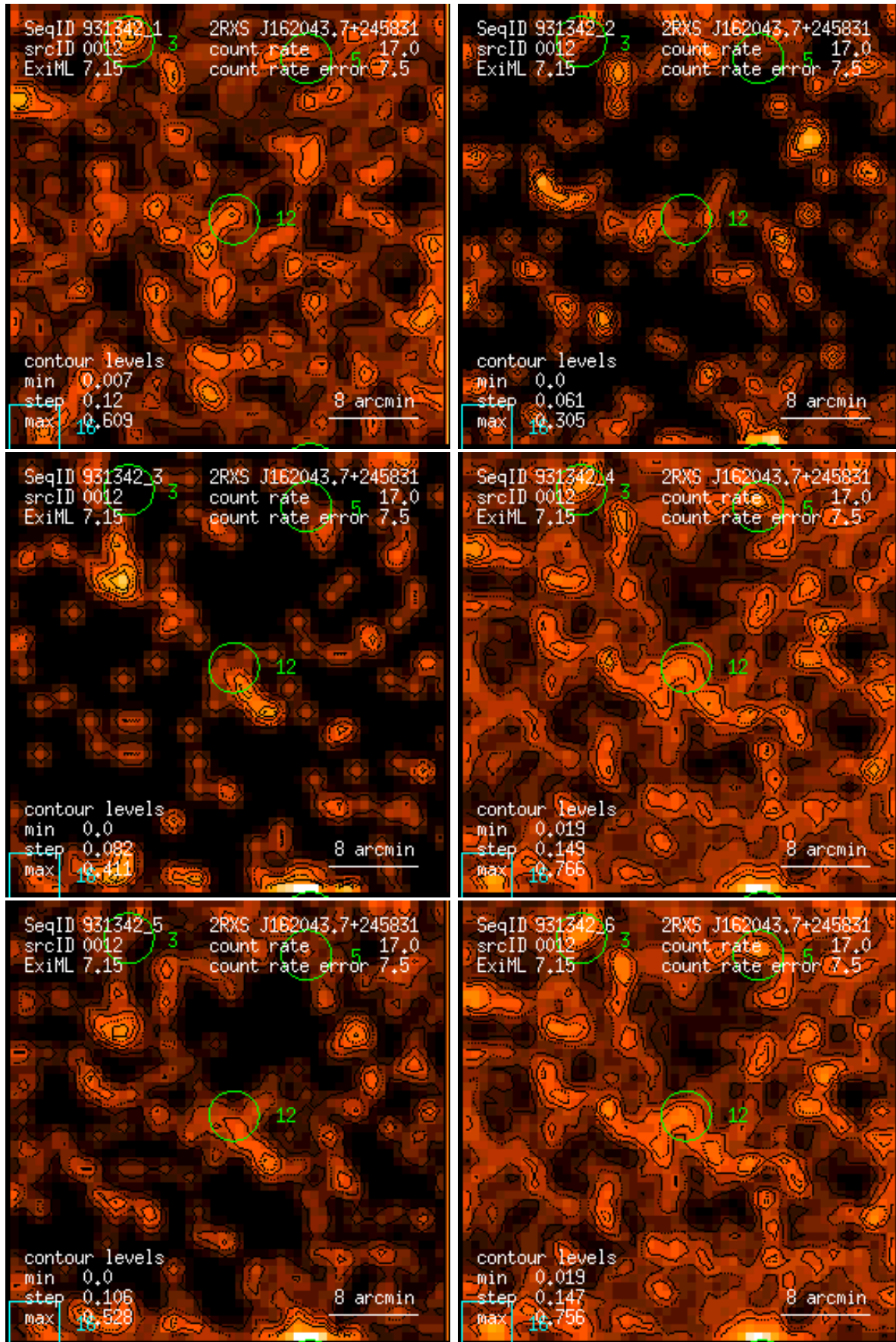
Figure 12: RASS 931342: detection 0012: band rate images, Gaussian filter: (1) PSPC channels 11 – 41, (2) 52 – 90, (3) 91 – 201, (4) 11 – 235, (5) 52 – 201, (6) 11 – 201. Broad band rates in counts/ks. Band rate contour levels in counts/ks/arcmin 2 .
