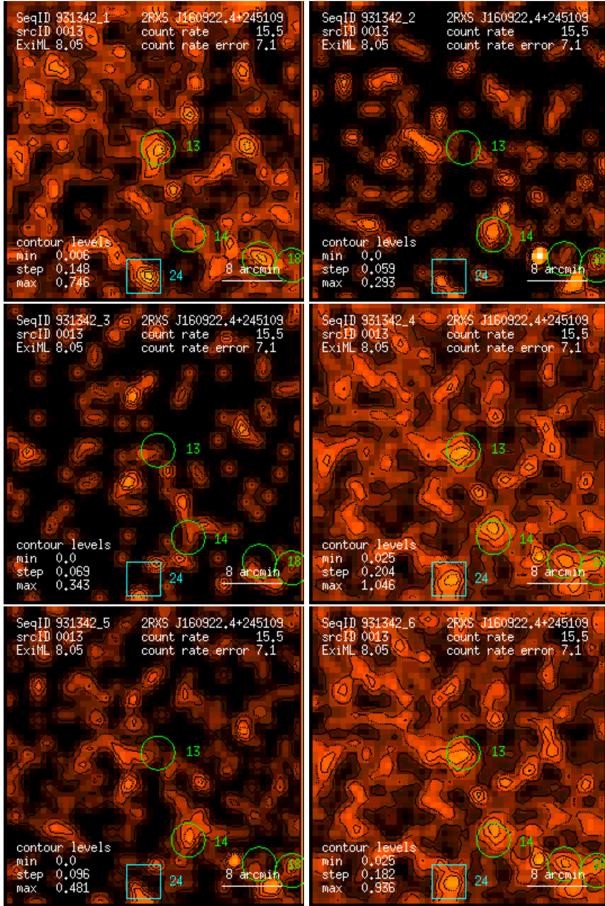
Figure 13: RASS 931342: detection 0013: band rate images, Gaussian filter: (1) PSPC channels 11 – 41, (2) 52 – 90, (3) 91 – 201, (4) 11 – 235, (5) 52 – 201, (6) 11 – 201. Broad band rates in counts/ks. Band rate contour levels in counts/ks/arcmin 2 .
