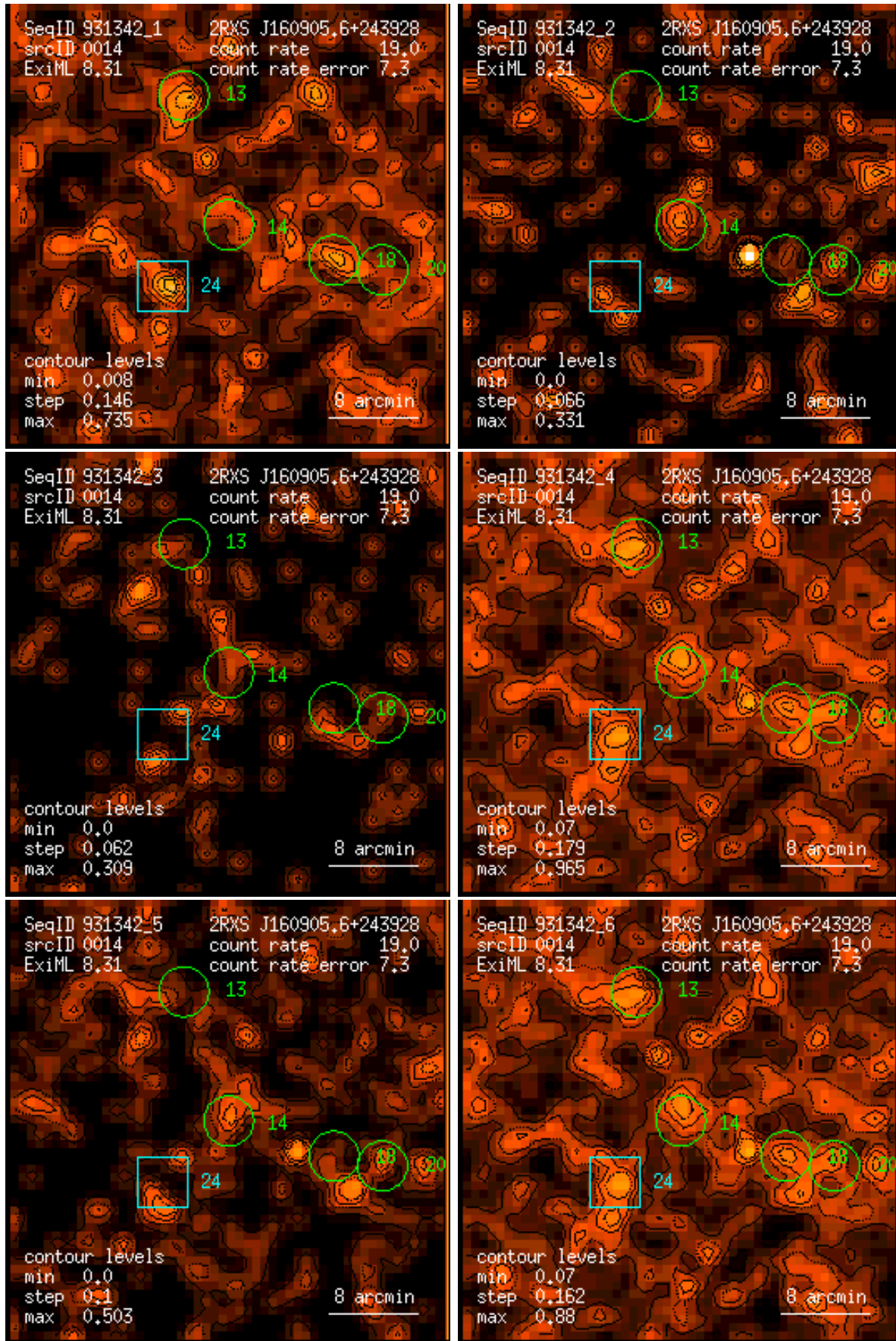
Figure 14: RASS 931342: detection 0014: band rate images, Gaussian filter: (1) PSPC channels 11 – 41, (2) 52 – 90, (3) 91 – 201, (4) 11 – 235, (5) 52 – 201, (6) 11 – 201. Broad band rates in counts/ks. Band rate contour levels in counts/ks/arcmin 2 .
