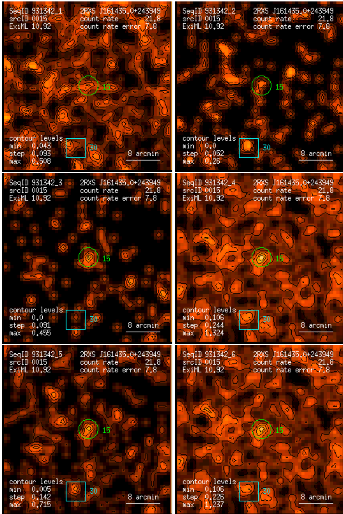
Figure 15: RASS 931342: detection 0015: band rate images, Gaussian filter: (1) PSPC channels 11 – 41, (2) 52 – 90, (3) 91 – 201, (4) 11 – 235, (5) 52 – 201, (6) 11 – 201. Broad band rates in counts/ks. Band rate contour levels in counts/ks/arcmin 2 .
