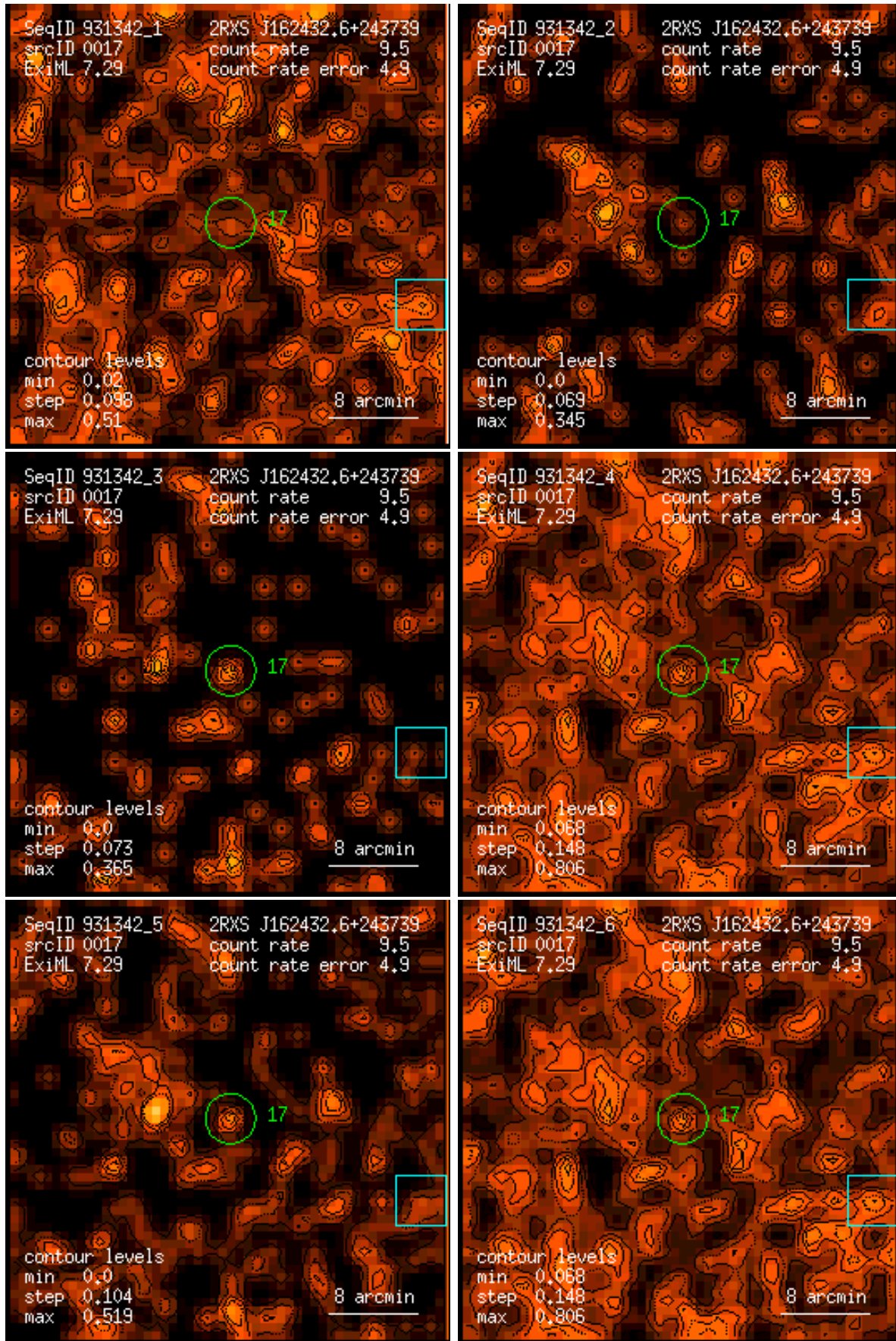
Figure 17: RASS 931342: detection 0017: band rate images, Gaussian filter: (1) PSPC channels 11 – 41, (2) 52 – 90, (3) 91 – 201, (4) 11 – 235, (5) 52 – 201, (6) 11 – 201. Broad band rates in counts/ks. Band rate contour levels in counts/ks/arcmin 2 .
