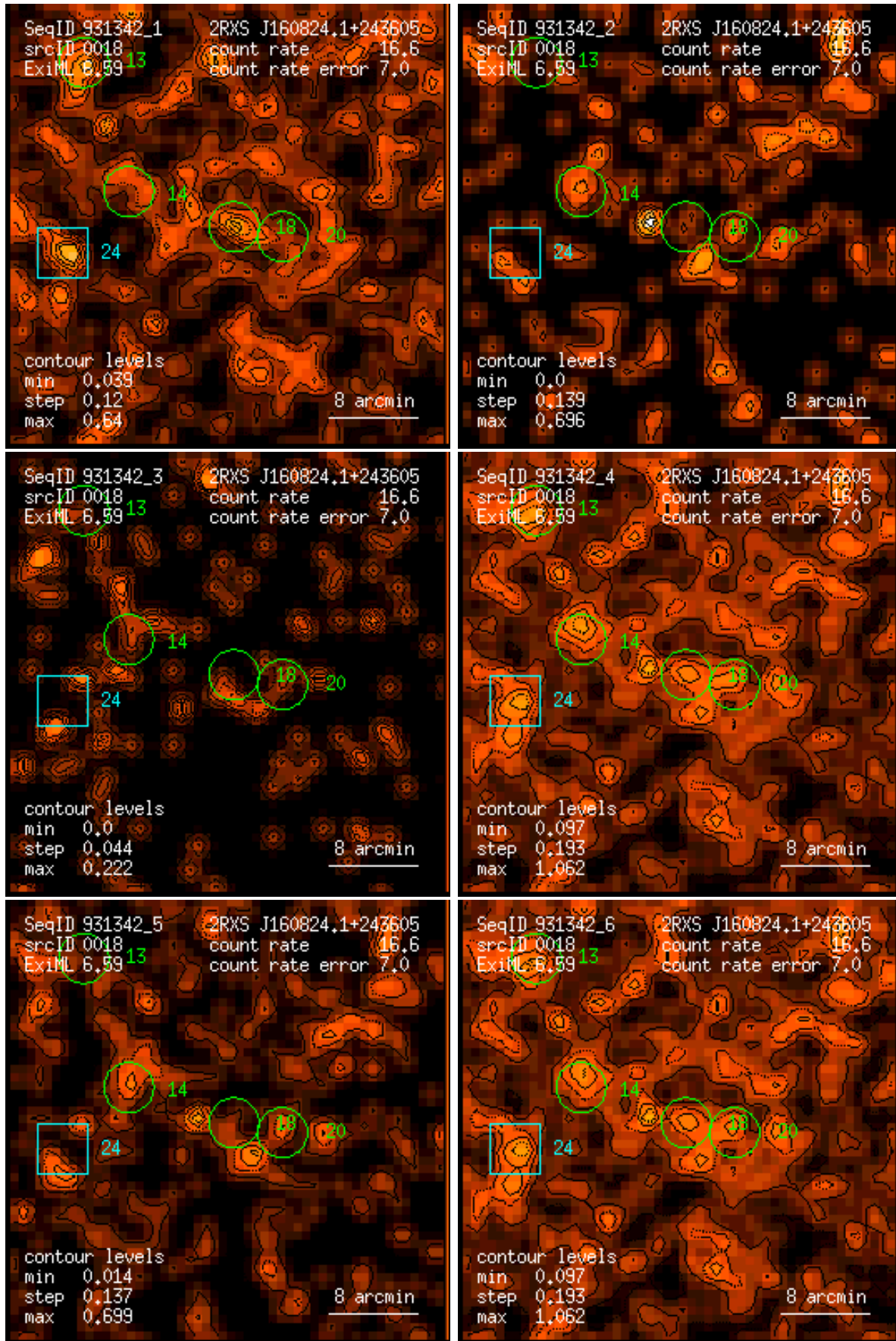
Figure 18: RASS 931342: detection 0018: band rate images, Gaussian filter: (1) PSPC channels 11 – 41, (2) 52 – 90, (3) 91 – 201, (4) 11 – 235, (5) 52 – 201, (6) 11 – 201. Broad band rates in counts/ks. Band rate contour levels in counts/ks/arcmin 2 .
