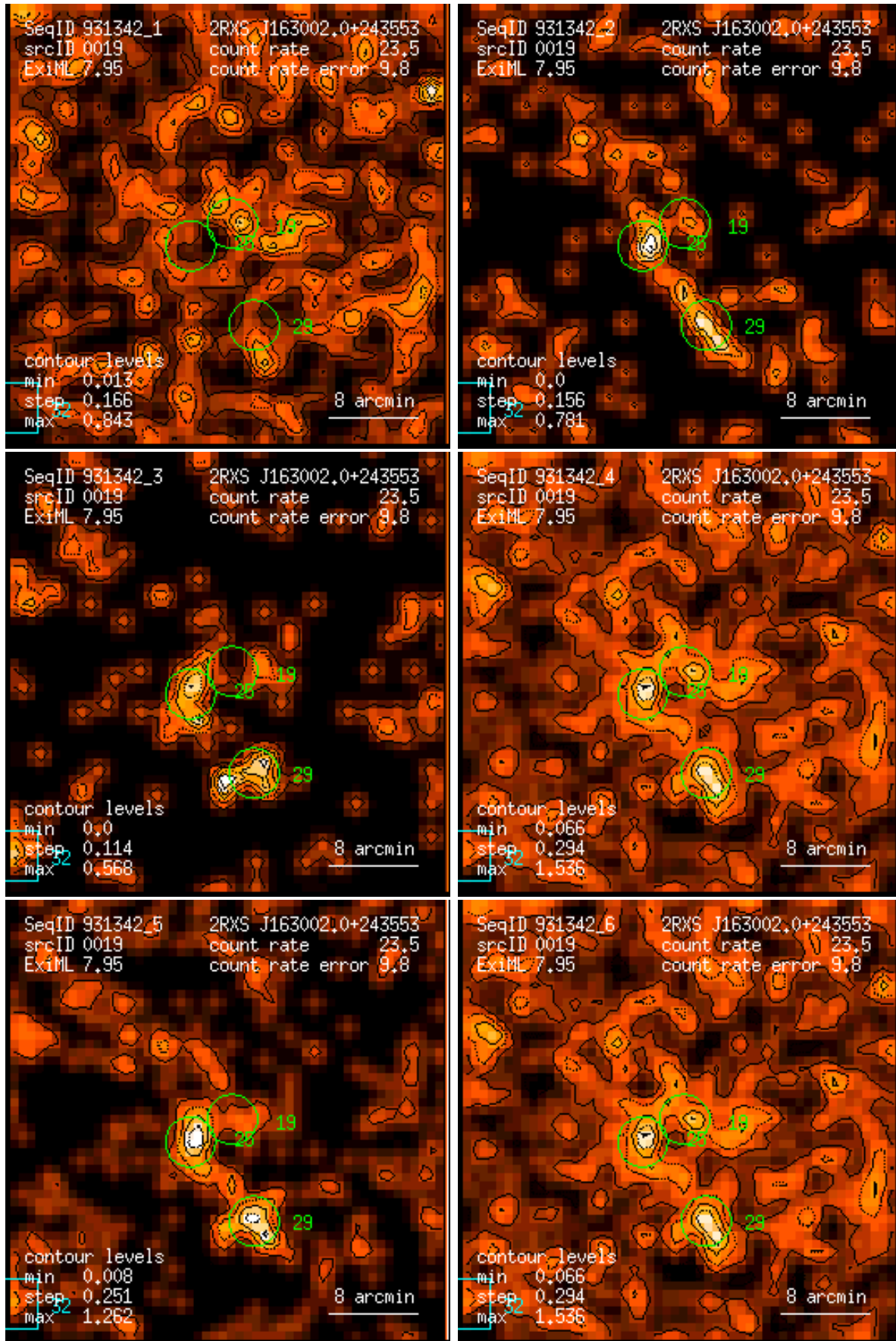
Figure 19: RASS 931342: detection 0019: band rate images, Gaussian filter: (1) PSPC channels 11 – 41, (2) 52 – 90, (3) 91 – 201, (4) 11 – 235, (5) 52 – 201, (6) 11 – 201. Broad band rates in counts/ks. Band rate contour levels in counts/ks/arcmin 2 .
