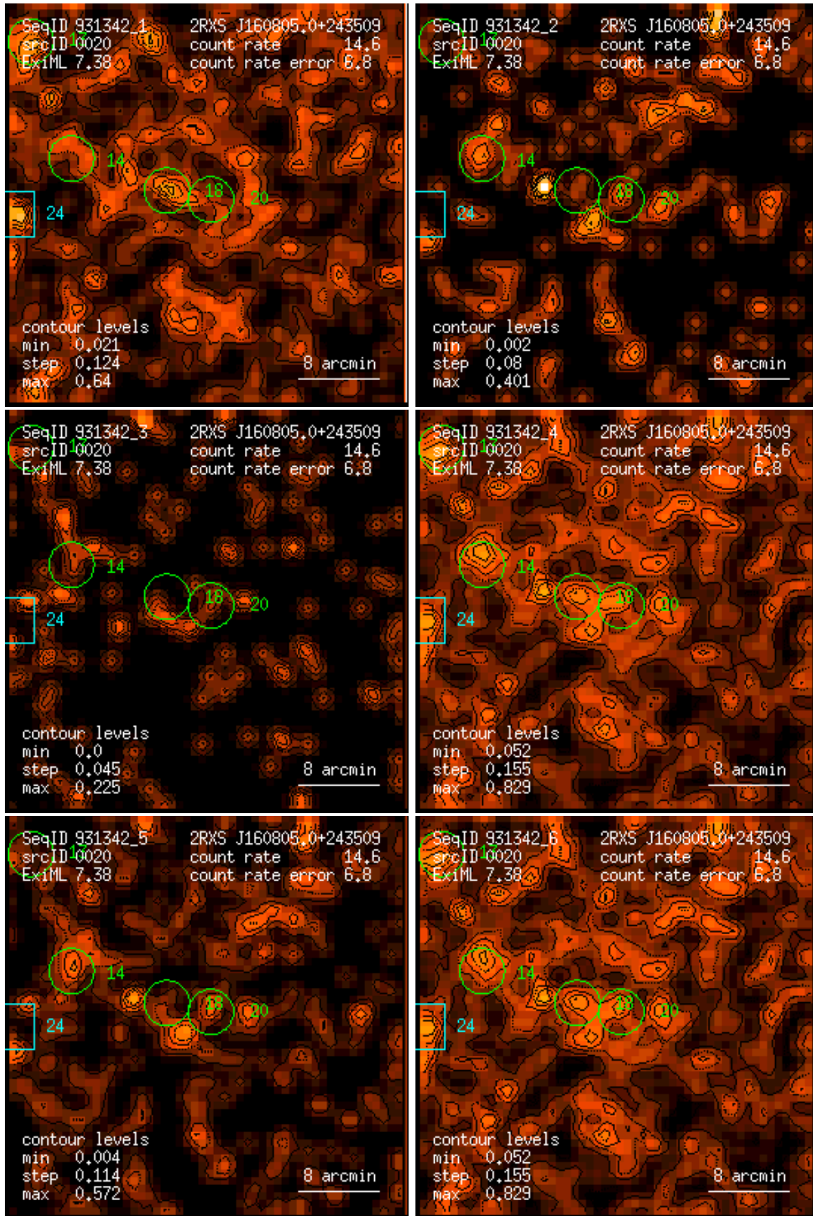
Figure 20: RASS 931342: detection 0020: band rate images, Gaussian filter: (1) PSPC channels 11 – 41, (2) 52 – 90, (3) 91 – 201, (4) 11 – 235, (5) 52 – 201, (6) 11 – 201. Broad band rates in counts/ks. Band rate contour levels in counts/ks/arcmin 2 .
