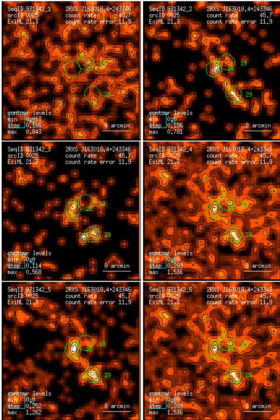
Figure 25: RASS 931342: detection 0025: band rate images, Gaussian filter: (1) PSPC channels 11 – 41, (2) 52 – 90, (3) 91 – 201, (4) 11 – 235, (5) 52 – 201, (6) 11 – 201. Broad band rates in counts/ks. Band rate contour levels in counts/ks/arcmin 2 .
