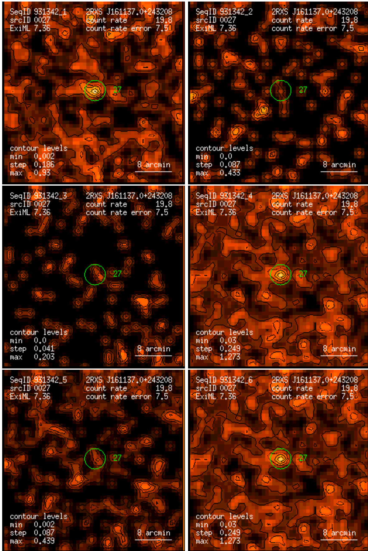
Figure 27: RASS 931342: detection 0027: band rate images, Gaussian filter: (1) PSPC channels 11 – 41, (2) 52 – 90, (3) 91 – 201, (4) 11 – 235, (5) 52 – 201, (6) 11 – 201. Broad band rates in counts/ks. Band rate contour levels in counts/ks/arcmin 2 .
