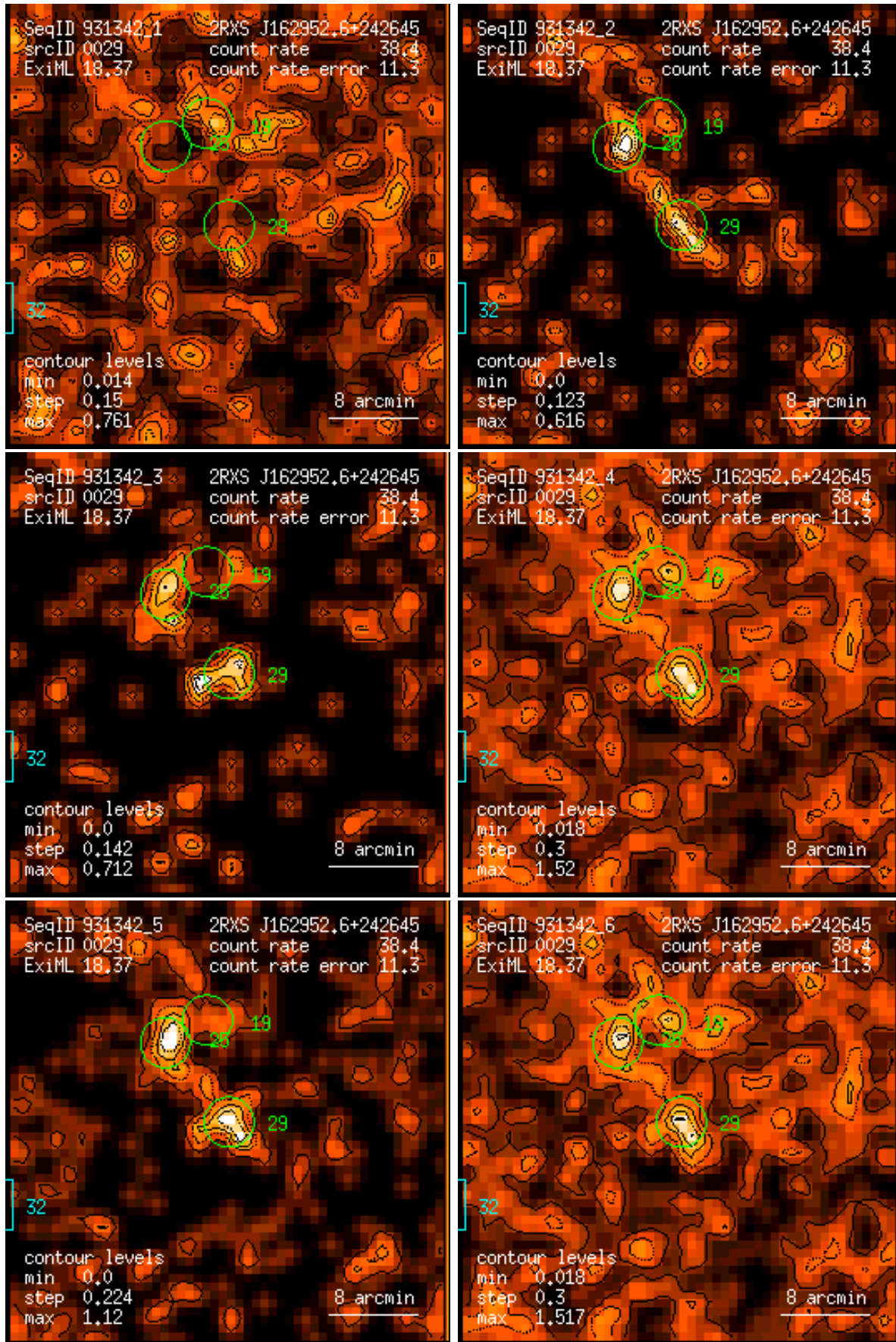
Figure 29: RASS 931342: detection 0029: band rate images, Gaussian filter: (1) PSPC channels 11 – 41, (2) 52 – 90, (3) 91 – 201, (4) 11 – 235, (5) 52 – 201, (6) 11 – 201. Broad band rates in counts/ks. Band rate contour levels in counts/ks/arcmin 2 .
