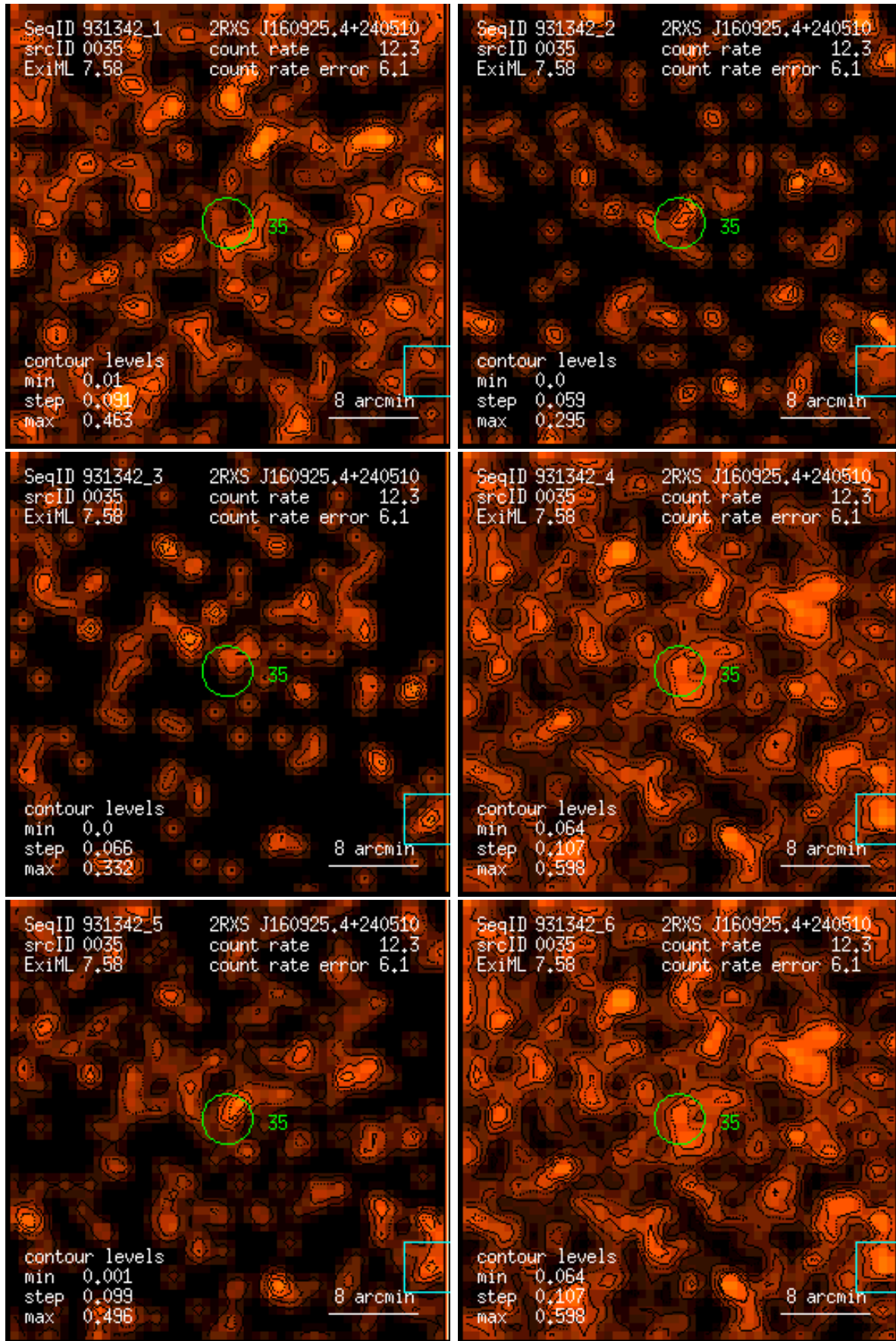
Figure 35: RASS 931342: detection 0035: band rate images, Gaussian filter: (1) PSPC channels 11 – 41, (2) 52 – 90, (3) 91 – 201, (4) 11 – 235, (5) 52 – 201, (6) 11 – 201. Broad band rates in counts/ks. Band rate contour levels in counts/ks/arcmin 2 .
