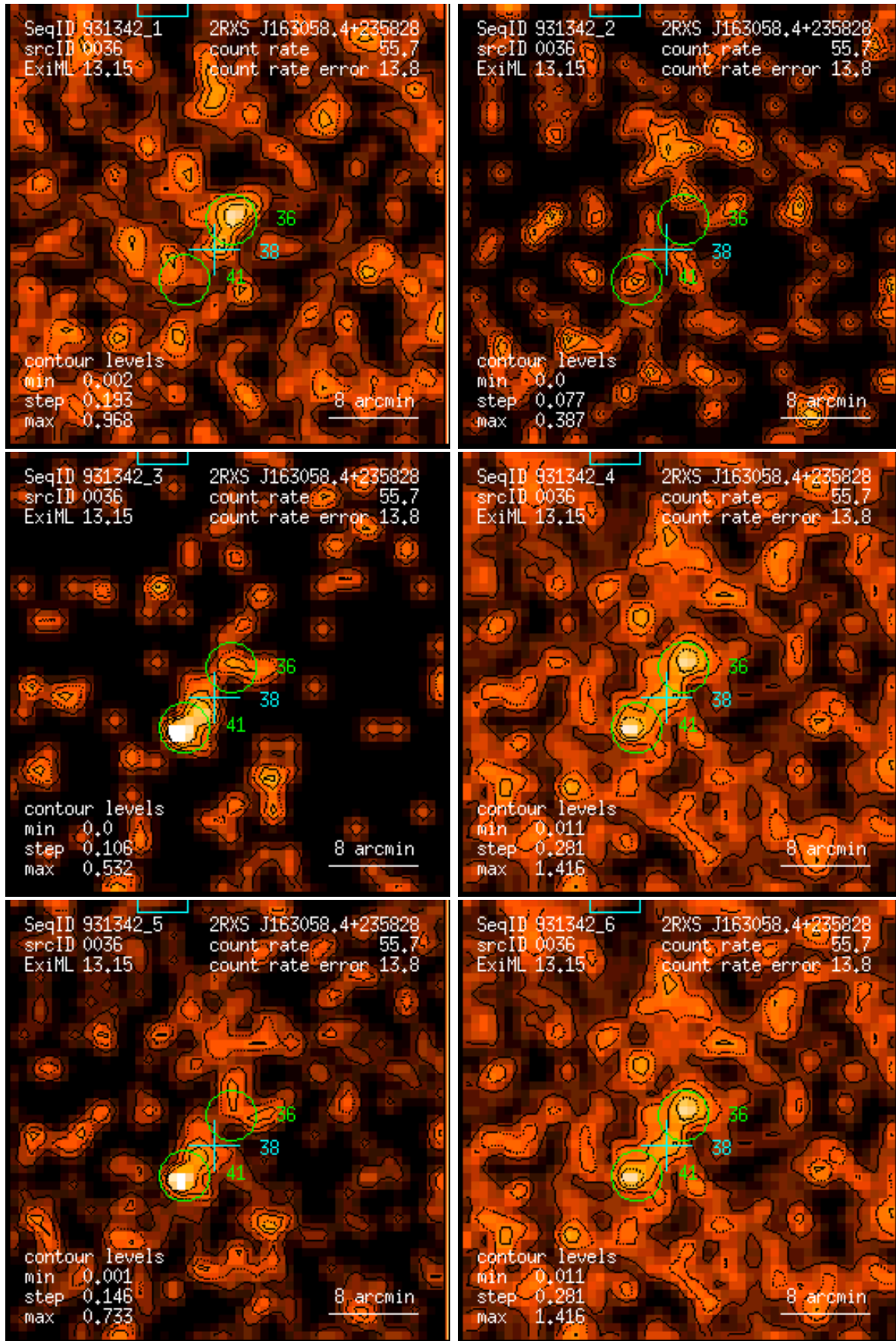
Figure 36: RASS 931342: detection 0036: band rate images, Gaussian filter: (1) PSPC channels 11 – 41, (2) 52 – 90, (3) 91 – 201, (4) 11 – 235, (5) 52 – 201, (6) 11 – 201. Broad band rates in counts/ks. Band rate contour levels in counts/ks/arcmin 2 .
