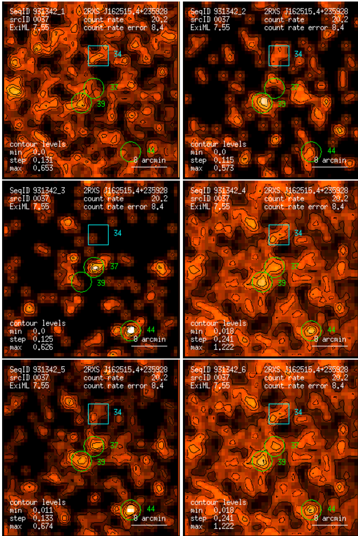
Figure 37: RASS 931342: detection 0037: band rate images, Gaussian filter: (1) PSPC channels 11 – 41, (2) 52 – 90, (3) 91 – 201, (4) 11 – 235, (5) 52 – 201, (6) 11 – 201. Broad band rates in counts/ks. Band rate contour levels in counts/ks/arcmin 2 .
