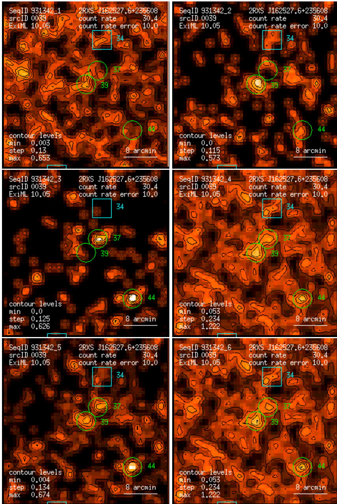
Figure 39: RASS 931342: detection 0039: band rate images, Gaussian filter: (1) PSPC channels 11 – 41, (2) 52 – 90, (3) 91 – 201, (4) 11 – 235, (5) 52 – 201, (6) 11 – 201. Broad band rates in counts/ks. Band rate contour levels in counts/ks/arcmin 2 .
