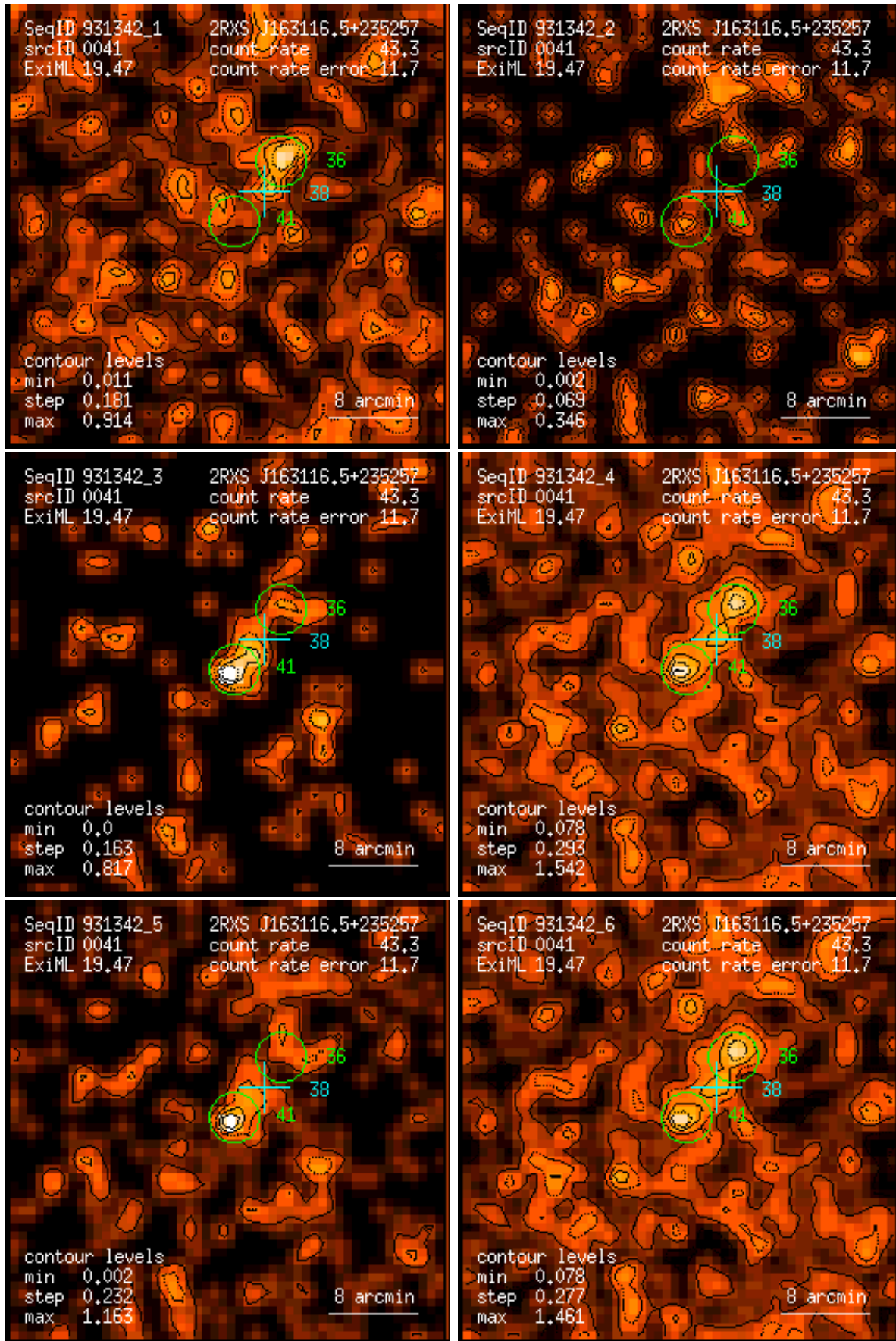
Figure 41: RASS 931342: detection 0041: band rate images, Gaussian filter: (1) PSPC channels 11 – 41, (2) 52 – 90, (3) 91 – 201, (4) 11 – 235, (5) 52 – 201, (6) 11 – 201. Broad band rates in counts/ks. Band rate contour levels in counts/ks/arcmin 2 .
