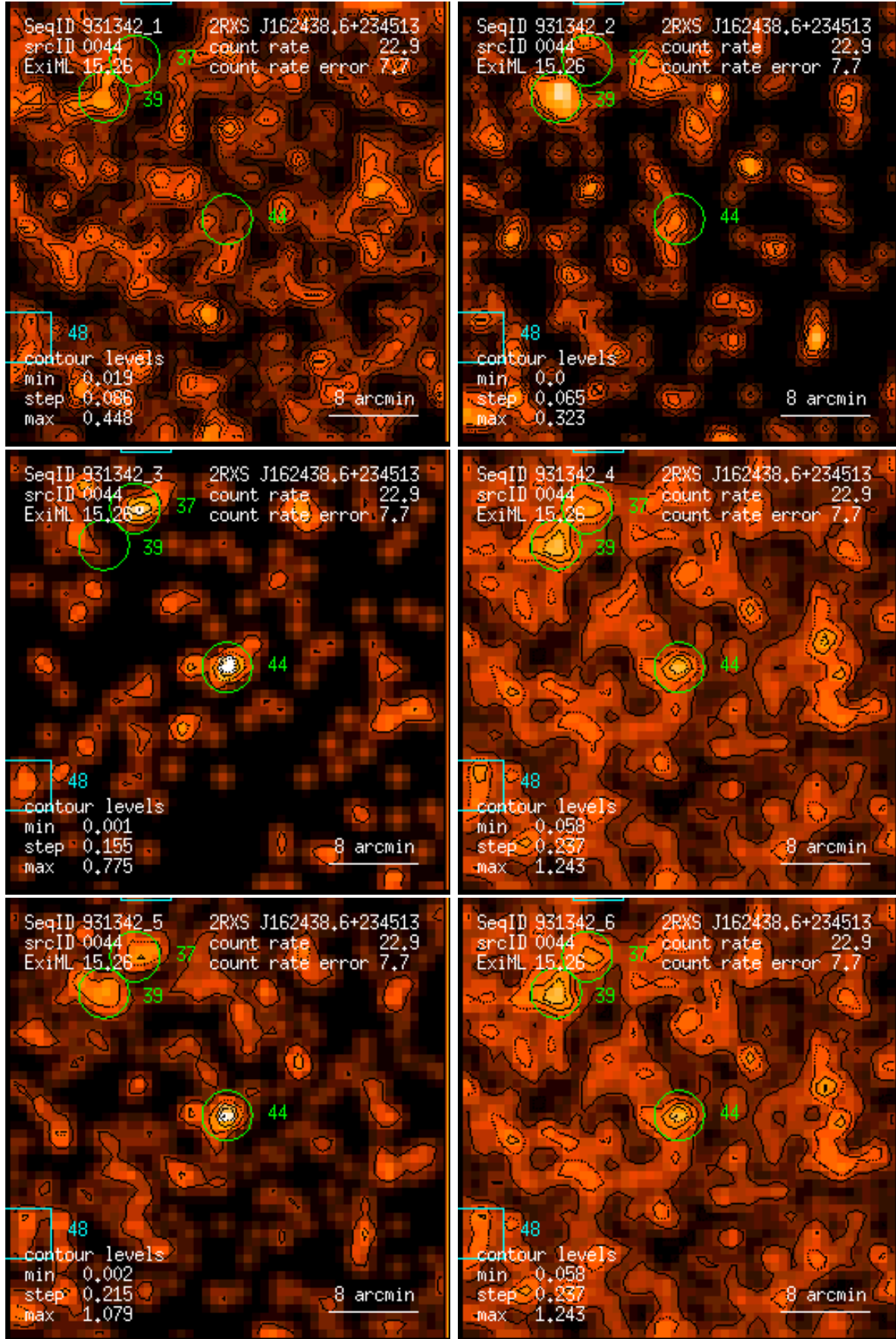
Figure 44: RASS 931342: detection 0044: band rate images, Gaussian filter: (1) PSPC channels 11 – 41, (2) 52 – 90, (3) 91 – 201, (4) 11 – 235, (5) 52 – 201, (6) 11 – 201. Broad band rates in counts/ks. Band rate contour levels in counts/ks/arcmin 2 .
