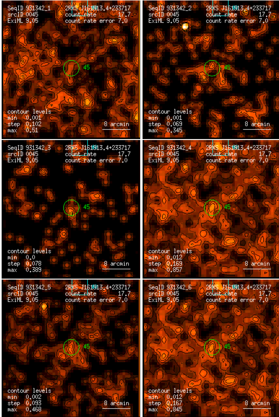
Figure 45: RASS 931342: detection 0045: band rate images, Gaussian filter: (1) PSPC channels 11 – 41, (2) 52 – 90, (3) 91 – 201, (4) 11 – 235, (5) 52 – 201, (6) 11 – 201. Broad band rates in counts/ks. Band rate contour levels in counts/ks/arcmin 2 .
