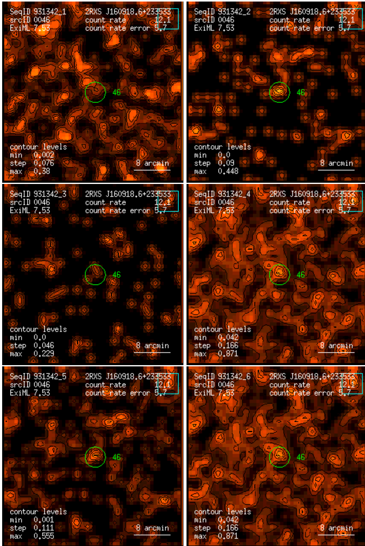
Figure 46: RASS 931342: detection 0046: band rate images, Gaussian filter: (1) PSPC channels 11 – 41, (2) 52 – 90, (3) 91 – 201, (4) 11 – 235, (5) 52 – 201, (6) 11 – 201. Broad band rates in counts/ks. Band rate contour levels in counts/ks/arcmin 2 .
