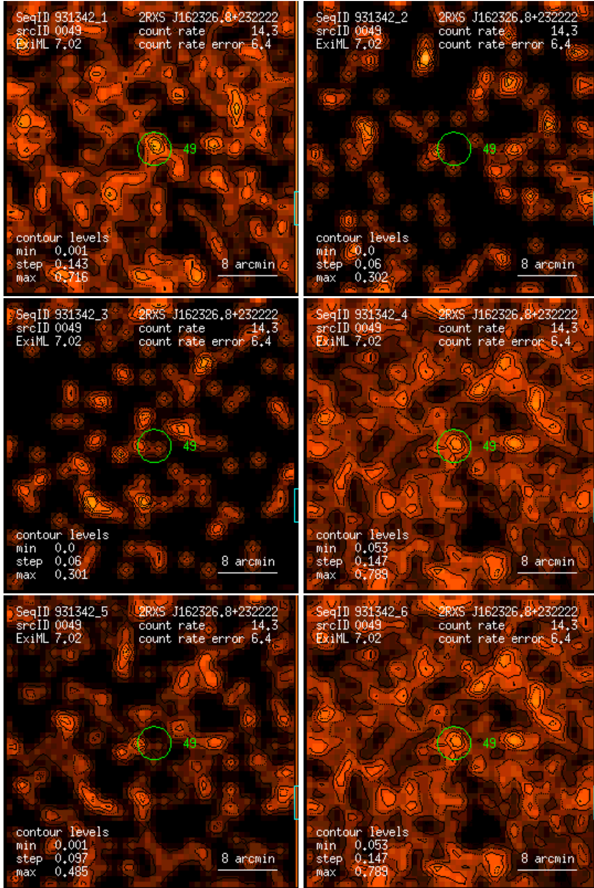
Figure 49: RASS 931342: detection 0049: band rate images, Gaussian filter: (1) PSPC channels 11 – 41, (2) 52 – 90, (3) 91 – 201, (4) 11 – 235, (5) 52 – 201, (6) 11 – 201. Broad band rates in counts/ks. Band rate contour levels in counts/ks/arcmin 2 .
