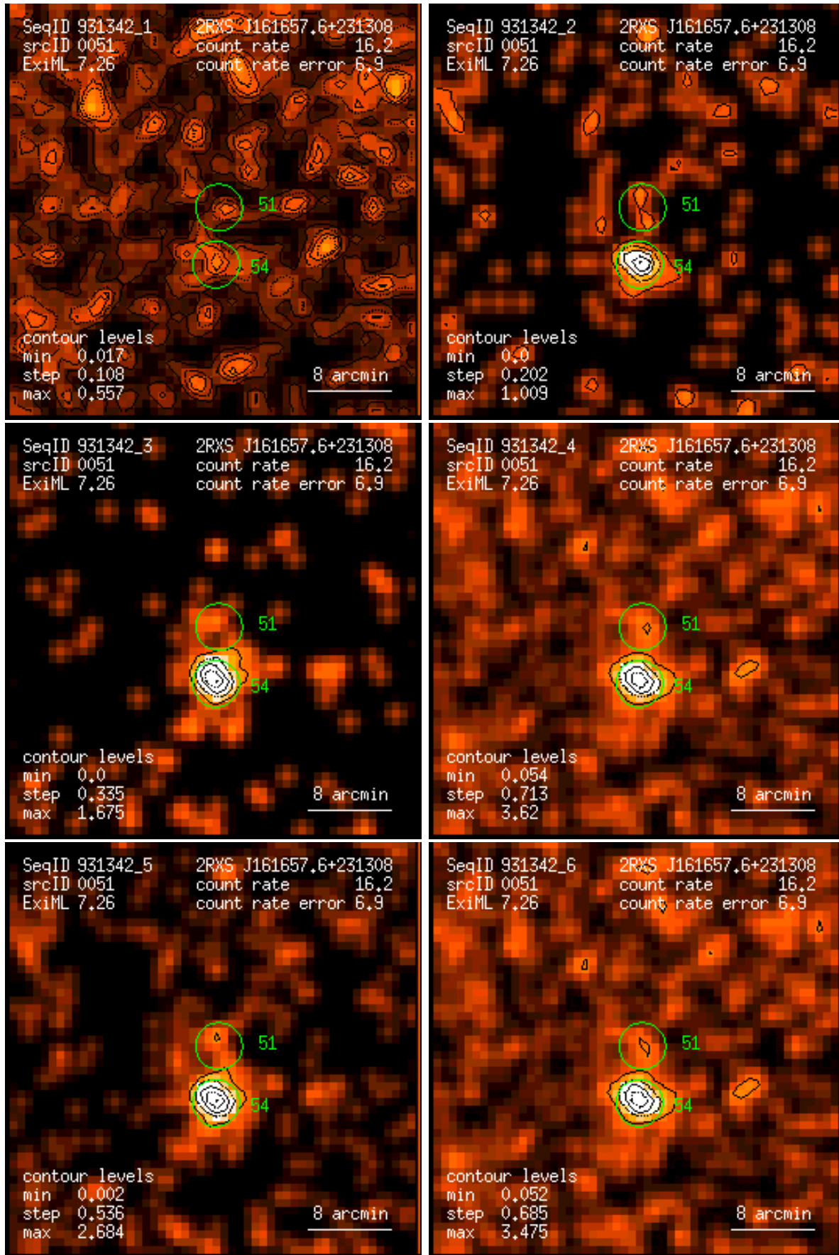
Figure 51: RASS 931342: detection 0051: band rate images, Gaussian filter: (1) PSPC channels 11 – 41, (2) 52 – 90, (3) 91 – 201, (4) 11 – 235, (5) 52 – 201, (6) 11 – 201. Broad band rates in counts/ks. Band rate contour levels in counts/ks/arcmin 2 .
