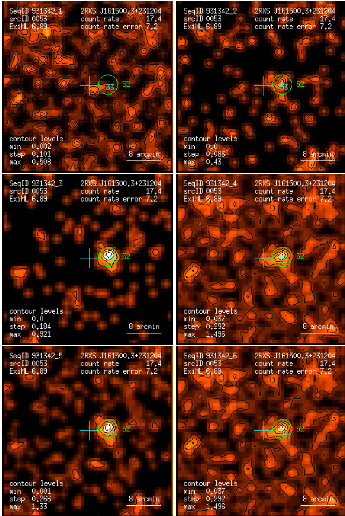
Figure 53: RASS 931342: detection 0053: band rate images, Gaussian filter: (1) PSPC channels 11 – 41, (2) 52 – 90, (3) 91 – 201, (4) 11 – 235, (5) 52 – 201, (6) 11 – 201. Broad band rates in counts/ks. Band rate contour levels in counts/ks/arcmin 2 .
