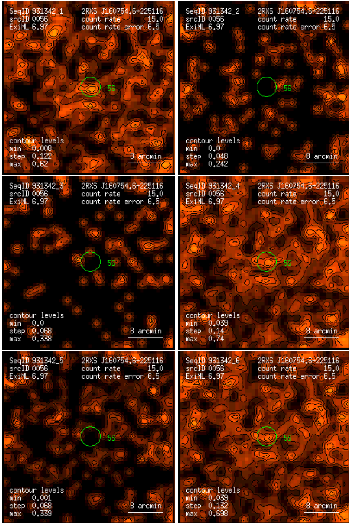
Figure 56: RASS 931342: detection 0056: band rate images, Gaussian filter: (1) PSPC channels 11 – 41, (2) 52 – 90, (3) 91 – 201, (4) 11 – 235, (5) 52 – 201, (6) 11 – 201. Broad band rates in counts/ks. Band rate contour levels in counts/ks/arcmin 2 .
