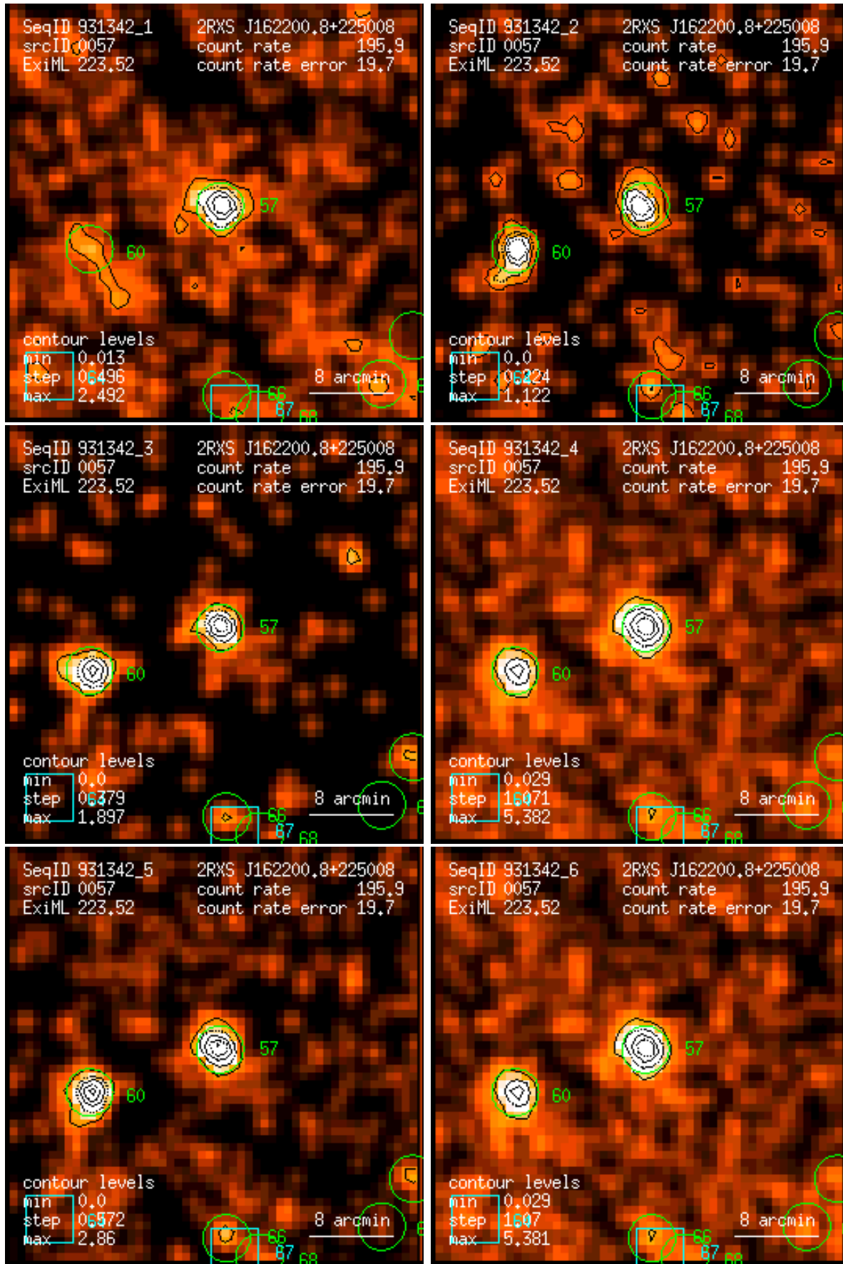
Figure 57: RASS 931342: detection 0057: band rate images, Gaussian filter: (1) PSPC channels 11 – 41, (2) 52 – 90, (3) 91 – 201, (4) 11 – 235, (5) 52 – 201, (6) 11 – 201. Broad band rates in counts/ks. Band rate contour levels in counts/ks/arcmin 2 .
