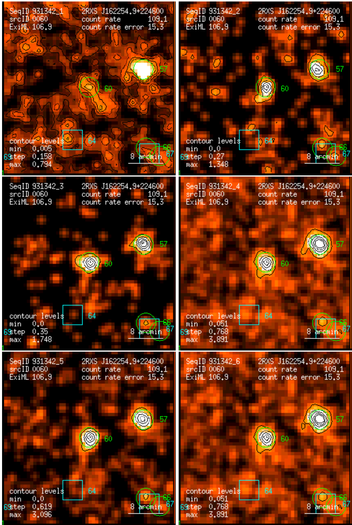
Figure 60: RASS 931342: detection 0060: band rate images, Gaussian filter: (1) PSPC channels 11 – 41, (2) 52 – 90, (3) 91 – 201, (4) 11 – 235, (5) 52 – 201, (6) 11 – 201. Broad band rates in counts/ks. Band rate contour levels in counts/ks/arcmin 2 .
