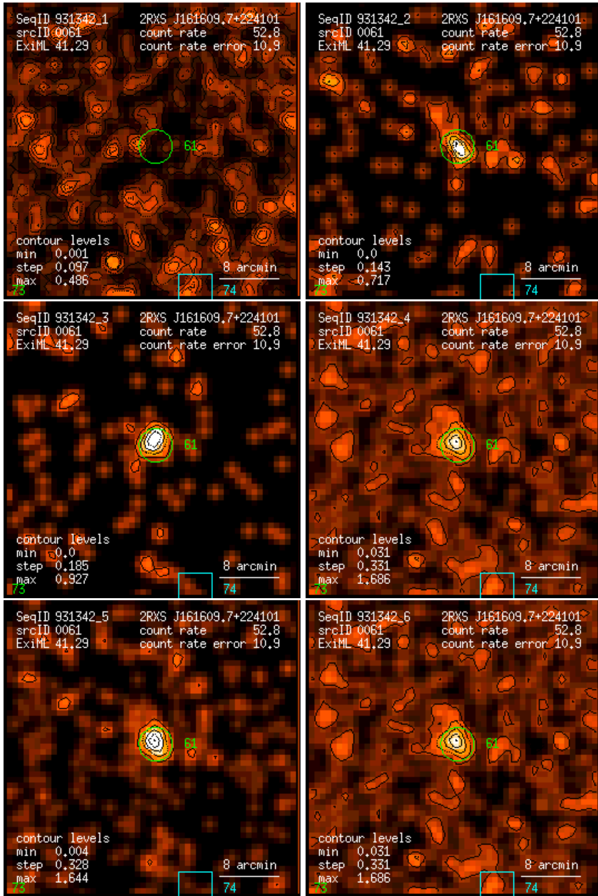
Figure 61: RASS 931342: detection 0061: band rate images, Gaussian filter: (1) PSPC channels 11 – 41, (2) 52 – 90, (3) 91 – 201, (4) 11 – 235, (5) 52 – 201, (6) 11 – 201. Broad band rates in counts/ks. Band rate contour levels in counts/ks/arcmin 2 .
