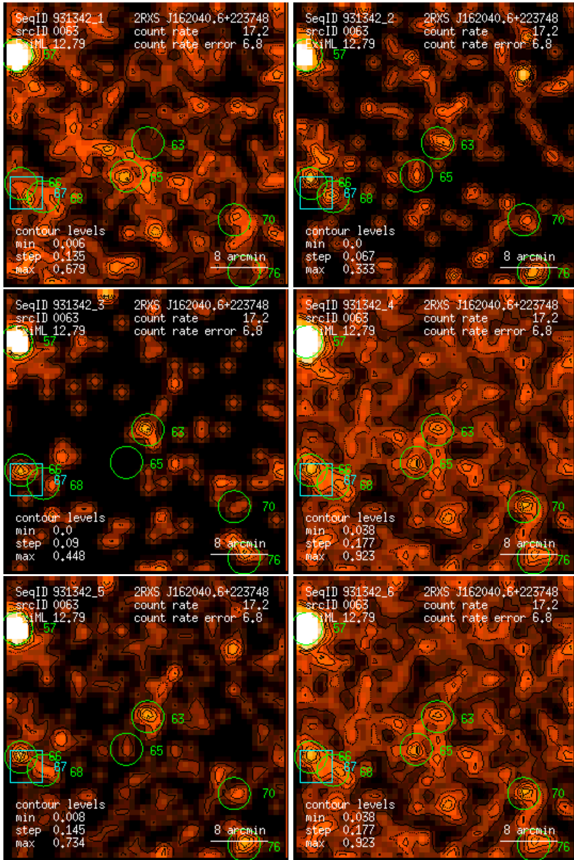
Figure 63: RASS 931342: detection 0063: band rate images, Gaussian filter: (1) PSPC channels 11 – 41, (2) 52 – 90, (3) 91 – 201, (4) 11 – 235, (5) 52 – 201, (6) 11 – 201. Broad band rates in counts/ks. Band rate contour levels in counts/ks/arcmin 2 .
