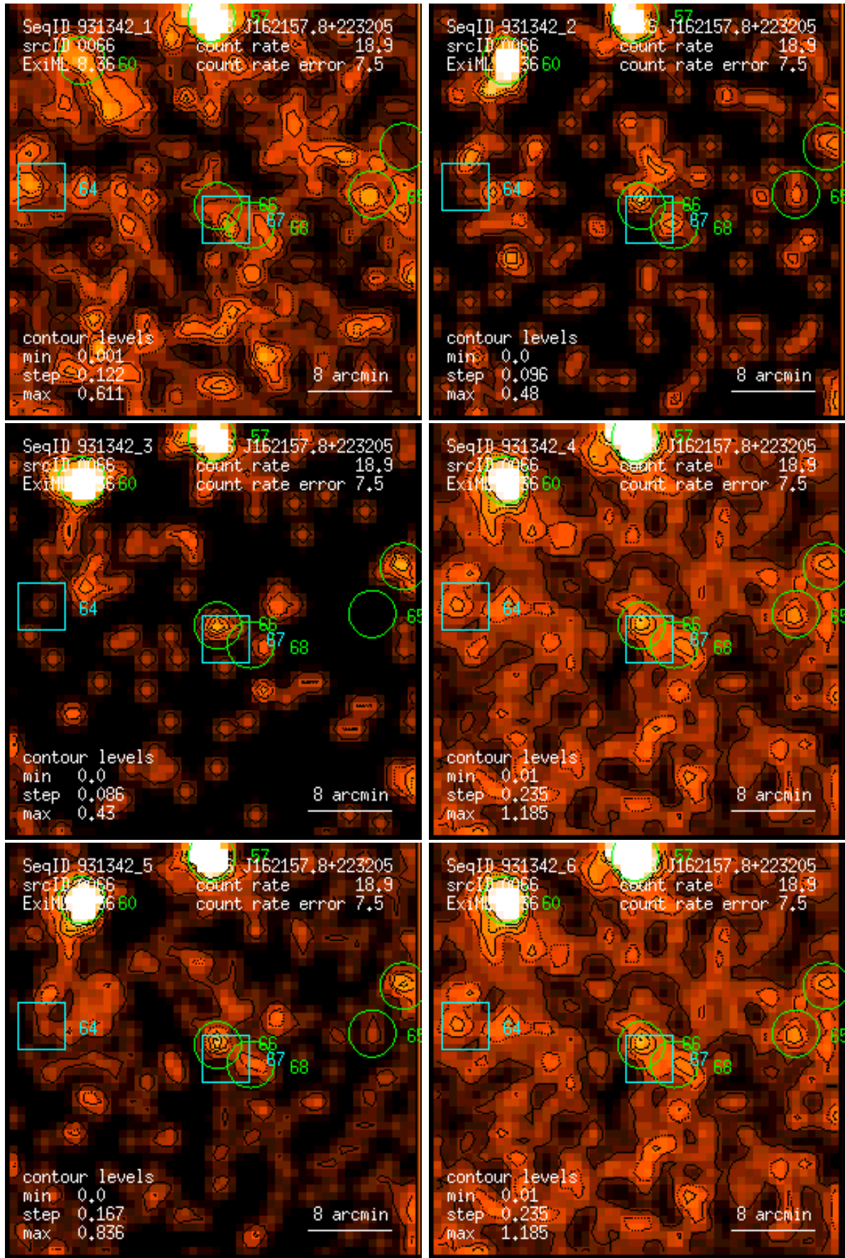
Figure 66: RASS 931342: detection 0066: band rate images, Gaussian filter: (1) PSPC channels 11 – 41, (2) 52 – 90, (3) 91 – 201, (4) 11 – 235, (5) 52 – 201, (6) 11 – 201. Broad band rates in counts/ks. Band rate contour levels in counts/ks/arcmin 2 .
