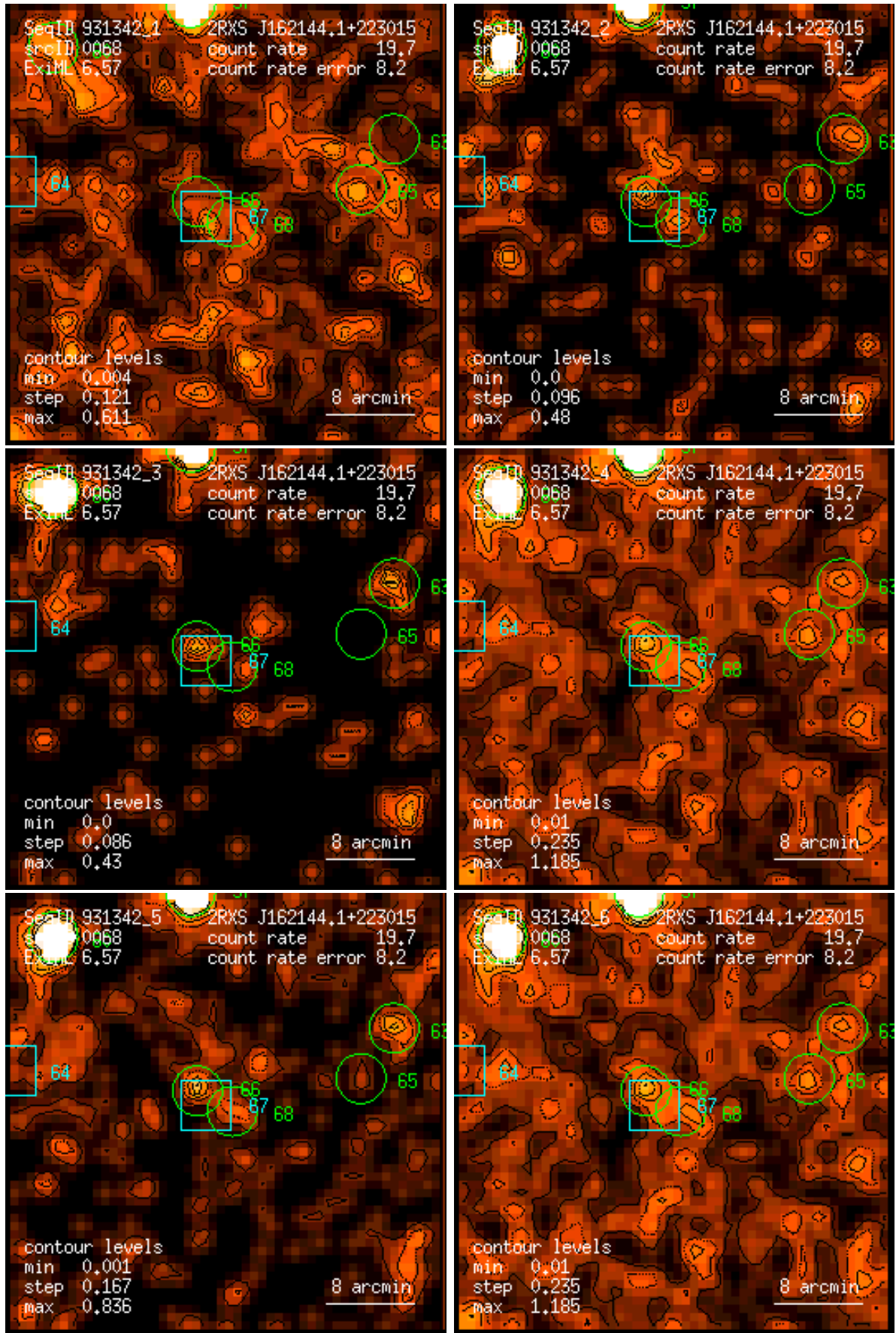
Figure 68: RASS 931342: detection 0068: band rate images, Gaussian filter: (1) PSPC channels 11 – 41, (2) 52 – 90, (3) 91 – 201, (4) 11 – 235, (5) 52 – 201, (6) 11 – 201. Broad band rates in counts/ks. Band rate contour levels in counts/ks/arcmin 2 .
