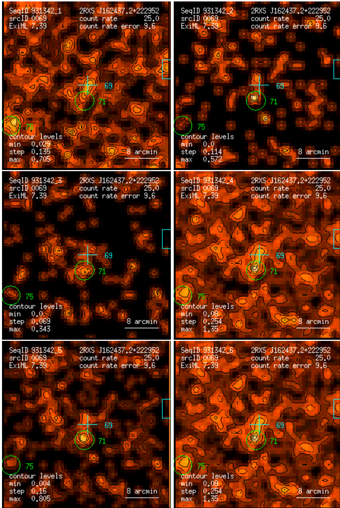
Figure 69: RASS 931342: detection 0069: band rate images, Gaussian filter: (1) PSPC channels 11 – 41, (2) 52 – 90, (3) 91 – 201, (4) 11 – 235, (5) 52 – 201, (6) 11 – 201. Broad band rates in counts/ks. Band rate contour levels in counts/ks/arcmin 2 .
