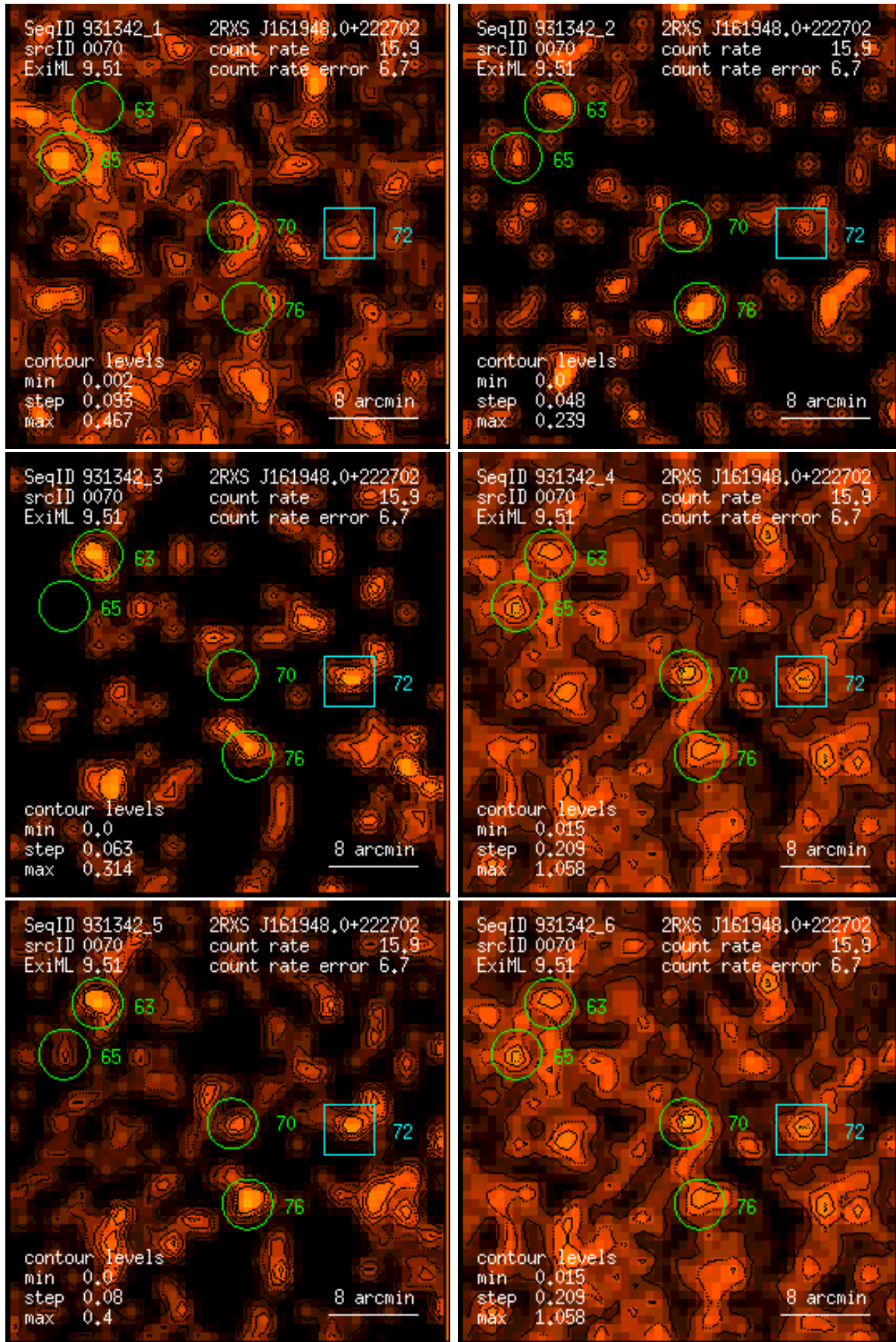
Figure 70: RASS 931342: detection 0070: band rate images, Gaussian filter: (1) PSPC channels 11 – 41, (2) 52 – 90, (3) 91 – 201, (4) 11 – 235, (5) 52 – 201, (6) 11 – 201. Broad band rates in counts/ks. Band rate contour levels in counts/ks/arcmin 2 .
