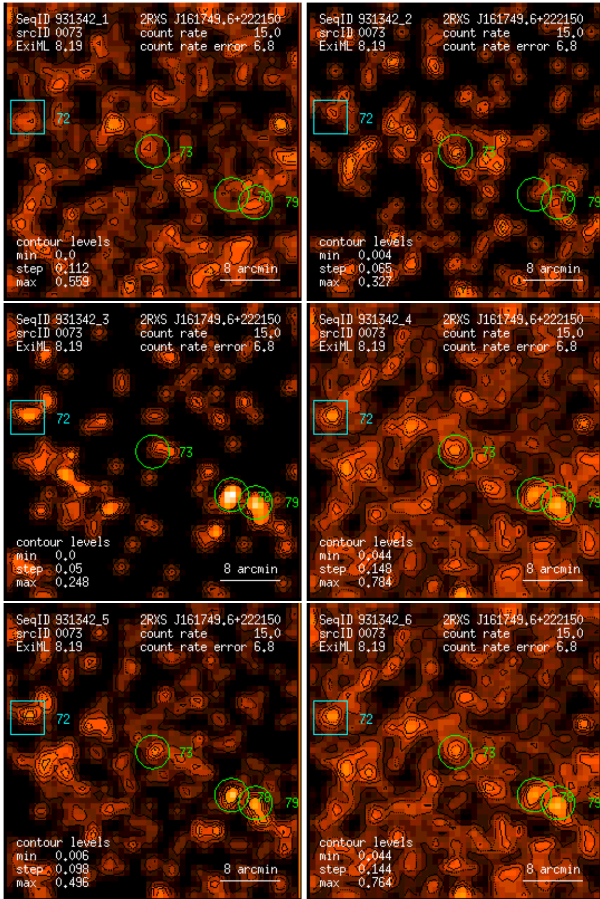
Figure 73: RASS 931342: detection 0073: band rate images, Gaussian filter: (1) PSPC channels 11 – 41, (2) 52 – 90, (3) 91 – 201, (4) 11 – 235, (5) 52 – 201, (6) 11 – 201. Broad band rates in counts/ks. Band rate contour levels in counts/ks/arcmin 2 .
