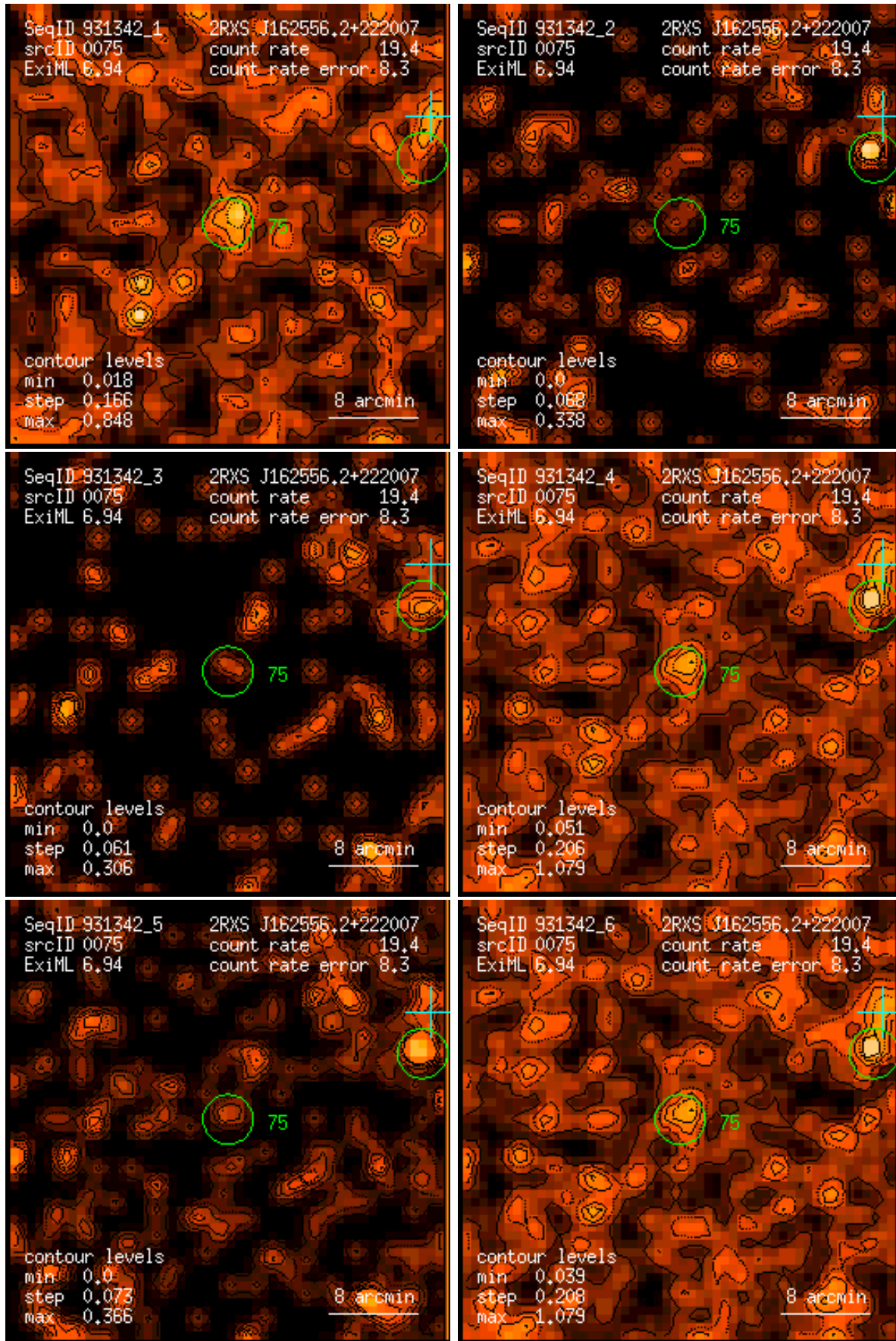
Figure 75: RASS 931342: detection 0075: band rate images, Gaussian filter: (1) PSPC channels 11 – 41, (2) 52 – 90, (3) 91 – 201, (4) 11 – 235, (5) 52 – 201, (6) 11 – 201. Broad band rates in counts/ks. Band rate contour levels in counts/ks/arcmin 2 .
