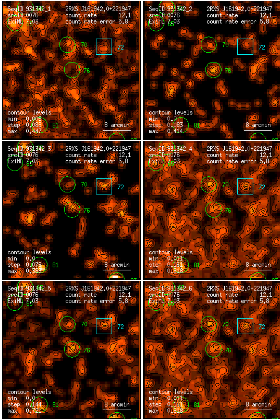
Figure 76: RASS 931342: detection 0076: band rate images, Gaussian filter: (1) PSPC channels 11 – 41, (2) 52 – 90, (3) 91 – 201, (4) 11 – 235, (5) 52 – 201, (6) 11 – 201. Broad band rates in counts/ks. Band rate contour levels in counts/ks/arcmin 2 .
