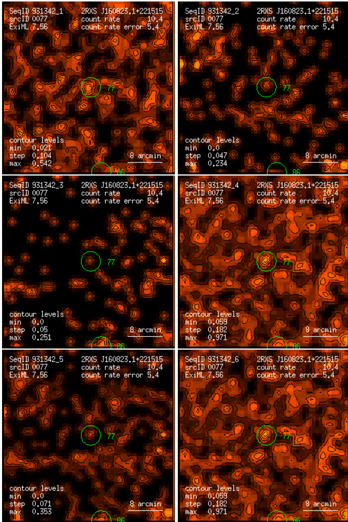
Figure 77: RASS 931342: detection 0077: band rate images, Gaussian filter: (1) PSPC channels 11 – 41, (2) 52 – 90, (3) 91 – 201, (4) 11 – 235, (5) 52 – 201, (6) 11 – 201. Broad band rates in counts/ks. Band rate contour levels in counts/ks/arcmin 2 .
