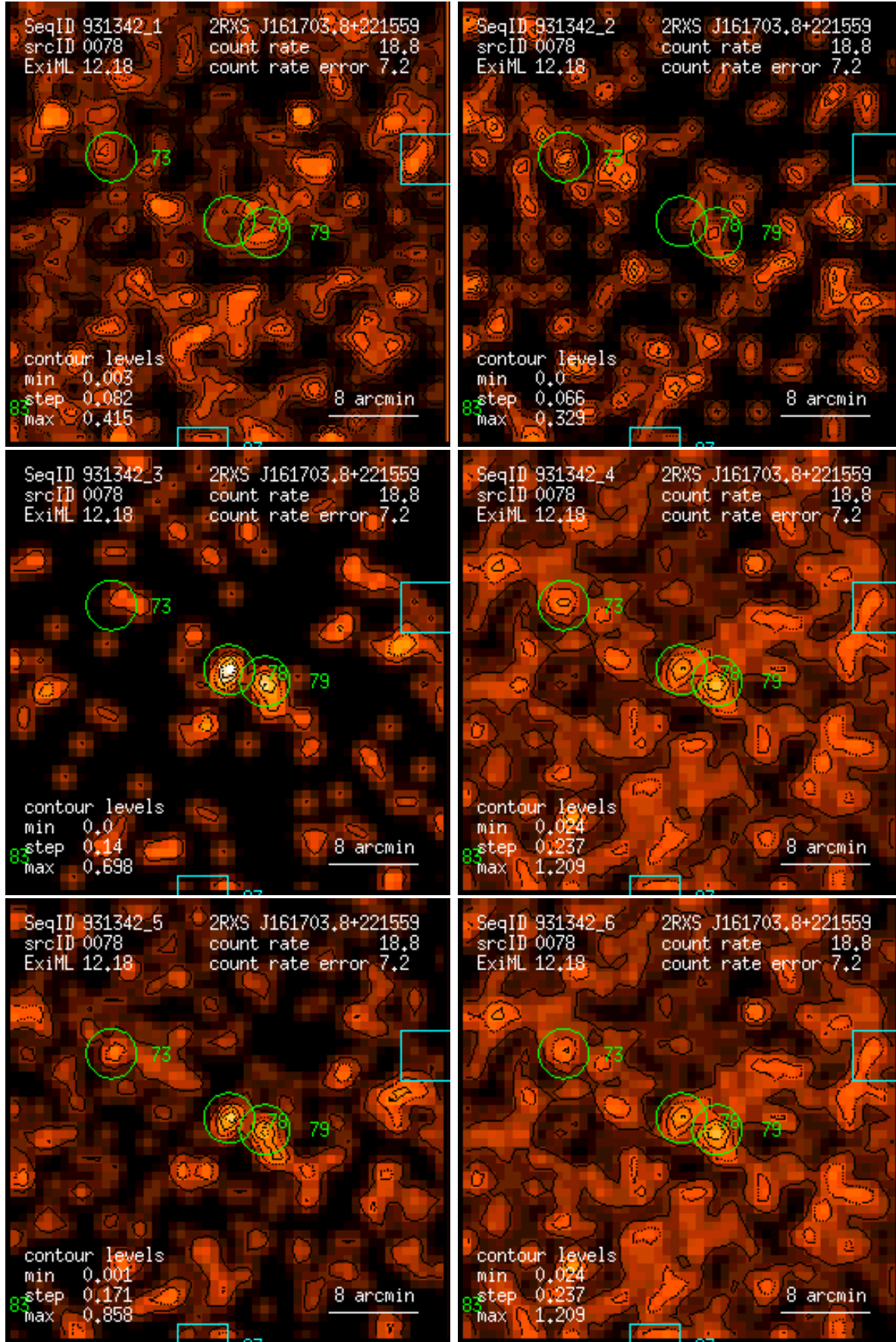
Figure 78: RASS 931342: detection 0078: band rate images, Gaussian filter: (1) PSPC channels 11 – 41, (2) 52 – 90, (3) 91 – 201, (4) 11 – 235, (5) 52 – 201, (6) 11 – 201. Broad band rates in counts/ks. Band rate contour levels in counts/ks/arcmin 2 .
