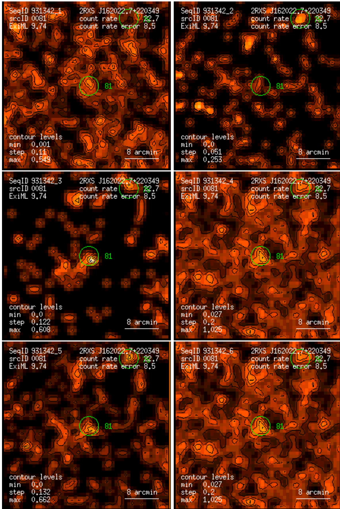
Figure 81: RASS 931342: detection 0081: band rate images, Gaussian filter: (1) PSPC channels 11 – 41, (2) 52 – 90, (3) 91 – 201, (4) 11 – 235, (5) 52 – 201, (6) 11 – 201. Broad band rates in counts/ks. Band rate contour levels in counts/ks/arcmin 2 .
