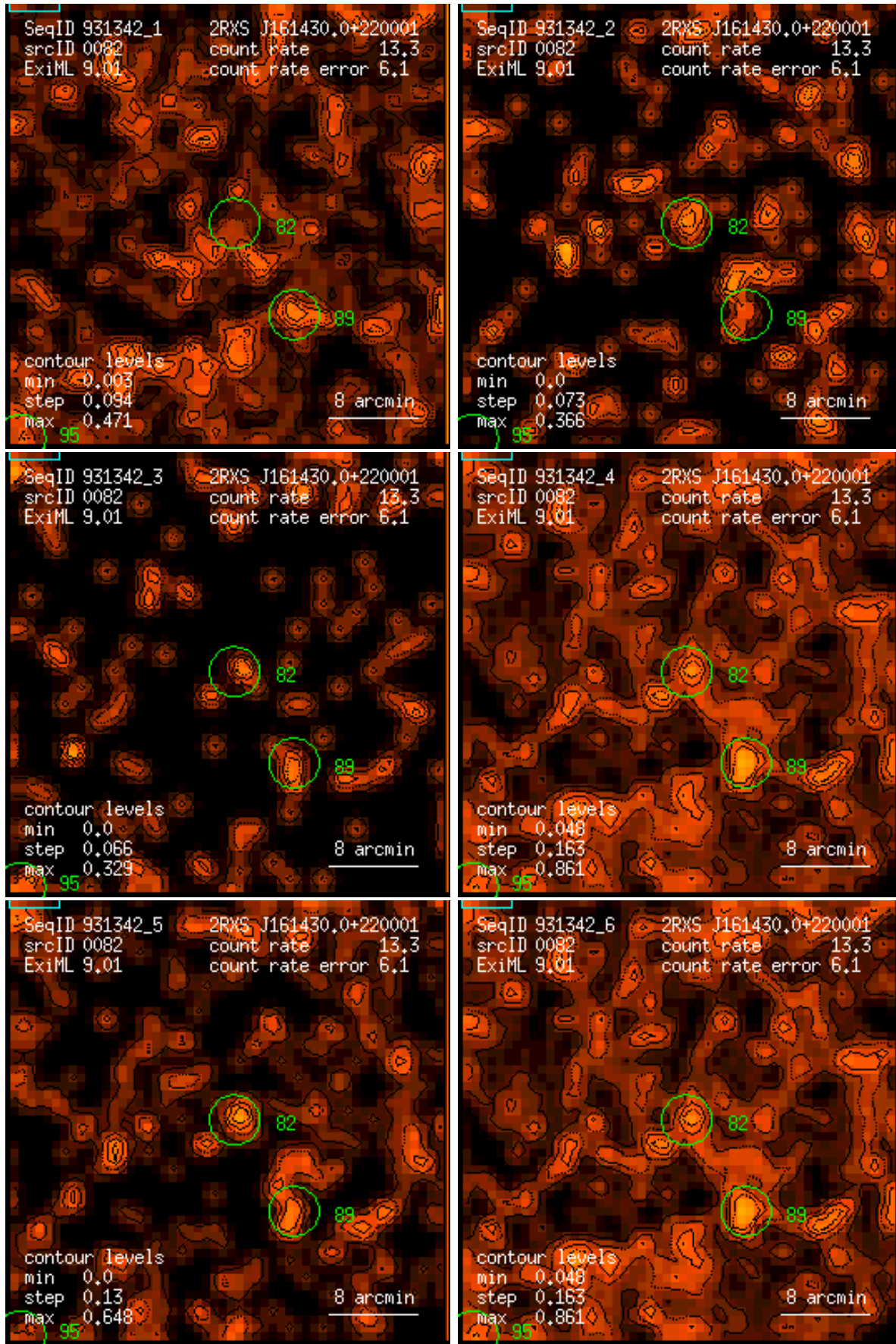
Figure 82: RASS 931342: detection 0082: band rate images, Gaussian filter: (1) PSPC channels 11 – 41, (2) 52 – 90, (3) 91 – 201, (4) 11 – 235, (5) 52 – 201, (6) 11 – 201. Broad band rates in counts/ks. Band rate contour levels in counts/ks/arcmin 2 .
