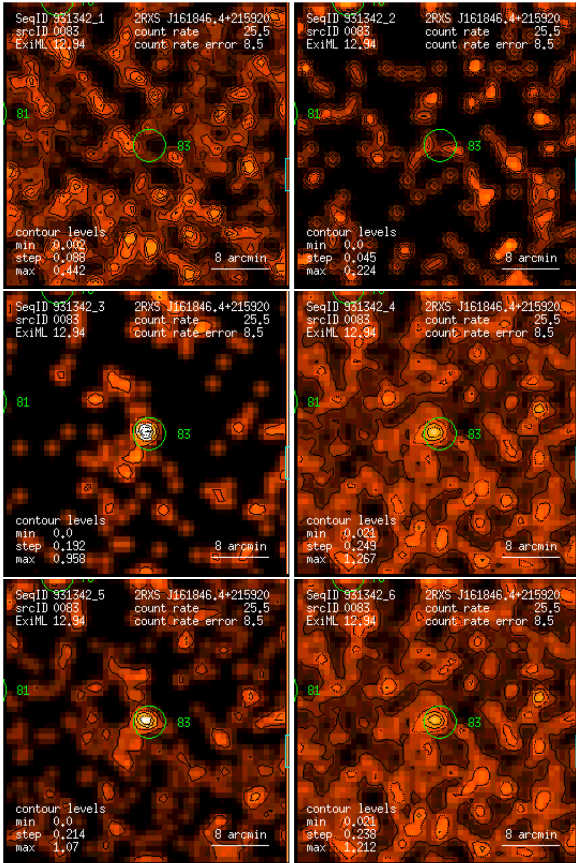
Figure 83: RASS 931342: detection 0083: band rate images, Gaussian filter: (1) PSPC channels 11 – 41, (2) 52 – 90, (3) 91 – 201, (4) 11 – 235, (5) 52 – 201, (6) 11 – 201. Broad band rates in counts/ks. Band rate contour levels in counts/ks/arcmin 2 .
