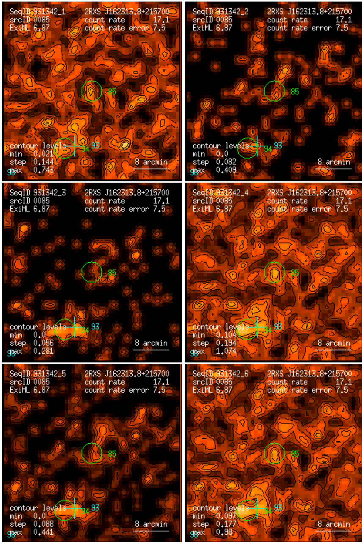
Figure 85: RASS 931342: detection 0085: band rate images, Gaussian filter: (1) PSPC channels 11 – 41, (2) 52 – 90, (3) 91 – 201, (4) 11 – 235, (5) 52 – 201, (6) 11 – 201. Broad band rates in counts/ks. Band rate contour levels in counts/ks/arcmin 2 .
