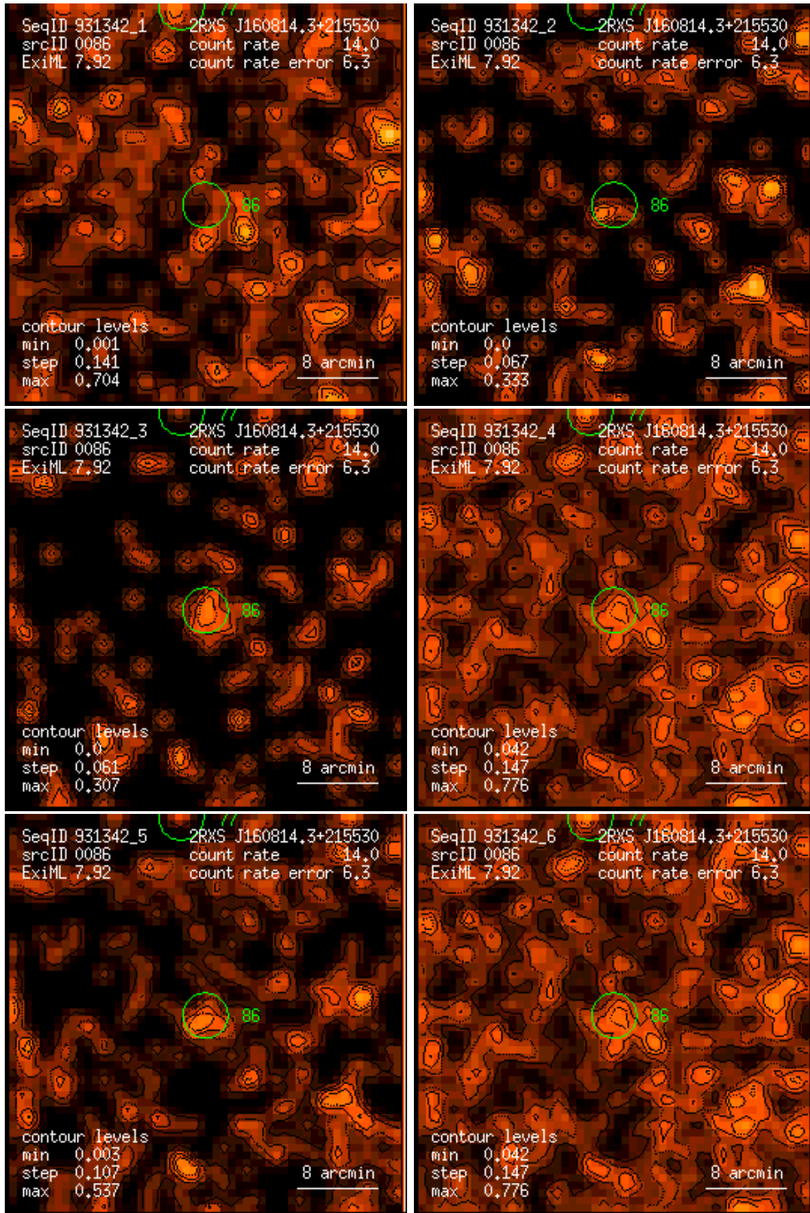
Figure 86: RASS 931342: detection 0086: band rate images, Gaussian filter: (1) PSPC channels 11 – 41, (2) 52 – 90, (3) 91 – 201, (4) 11 – 235, (5) 52 – 201, (6) 11 – 201. Broad band rates in counts/ks. Band rate contour levels in counts/ks/arcmin 2 .
