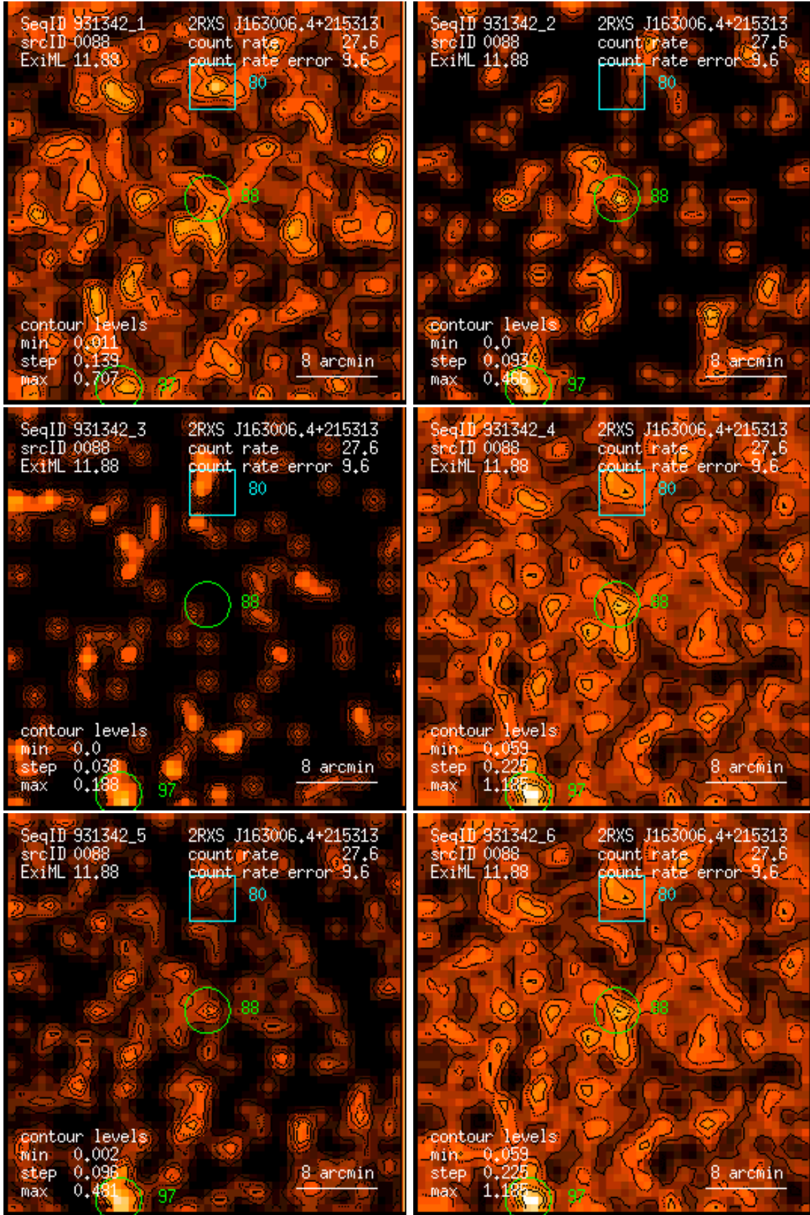
Figure 88: RASS 931342: detection 0088: band rate images, Gaussian filter: (1) PSPC channels 11 – 41, (2) 52 – 90, (3) 91 – 201, (4) 11 – 235, (5) 52 – 201, (6) 11 – 201. Broad band rates in counts/ks. Band rate contour levels in counts/ks/arcmin 2 .
